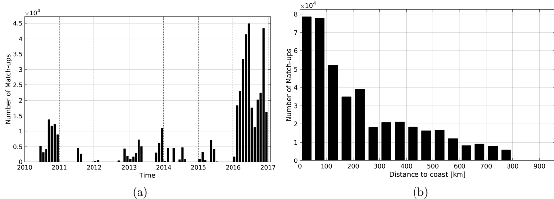
Figure 1: Number of match-ups between TSG-GOSUD-Sailing-ship and SMOS-L3-CATDS-CECOS-LOCEAN-V2-9DAYS-25KM SSS as a function of time (a) and as function of the distance to coast (b) over the SMOS coastal zone ( \leq 800 km) 60N-60S Pi-MEP region and for the full satellite product period.
