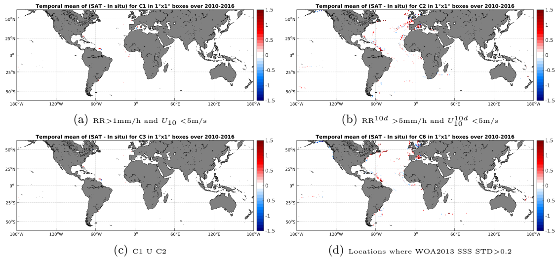
Figure 12: Temporal mean gridded over spatial boxes of size 1^\circ \times 1^\circ of \Delta SSS (SMOS-L3-CATDS-CECOS-LOCEAN-V2-9DAYS-25KM - TSG-GOSUD-Sailing-ship) for 4 different subdatasets corresponding to: RR > 1\text{mm/h} and U_{10} < 5\text{m/s} (a), RR^{10d} > 5\text{mm/h} and U_{10}^{10d} < 5\text{m/s} (b), C1 U C2 (c), Locations where WOA2013 SSS STD > 0.2 (d).
