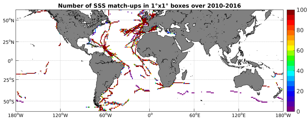
Figure 4: Number of SSS match-ups between TSG-GOSUD-Sailing-ship SSS and the SMOS-L3-CATDS-CECOS-LOCEAN-V2-9DAYS-25KM SSS product for the SMOS coastal zone ( \pm 800\text{km} ) 60N-60S Pi-MEP region over 1^\circ \times 1^\circ boxes and for the full satellite product period.
