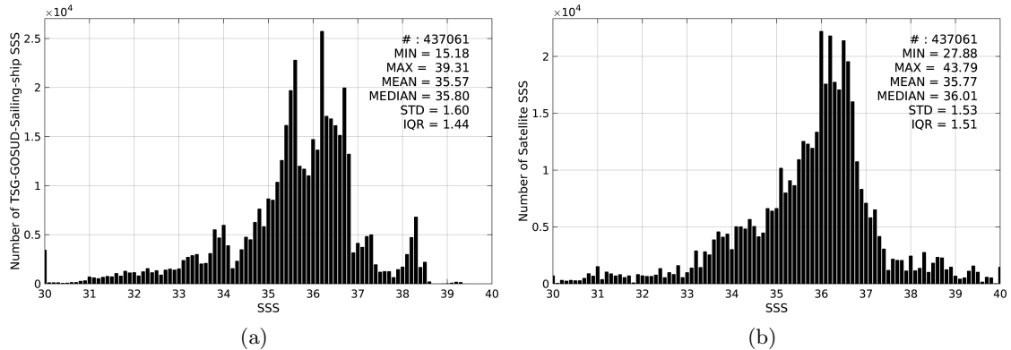
Figure 2: Histograms of SSS from TSG-GOSUD-Sailing-ship (a) and SMOS-L3-CATDS-CECOS-LOCEAN-V2-9DAYS-25KM (b) considering all match-up pairs per bins of 0.1 over the SMOS coastal zone ( \leq 800 km) 60N-60S Pi-MEP region and for the full satellite product period.
