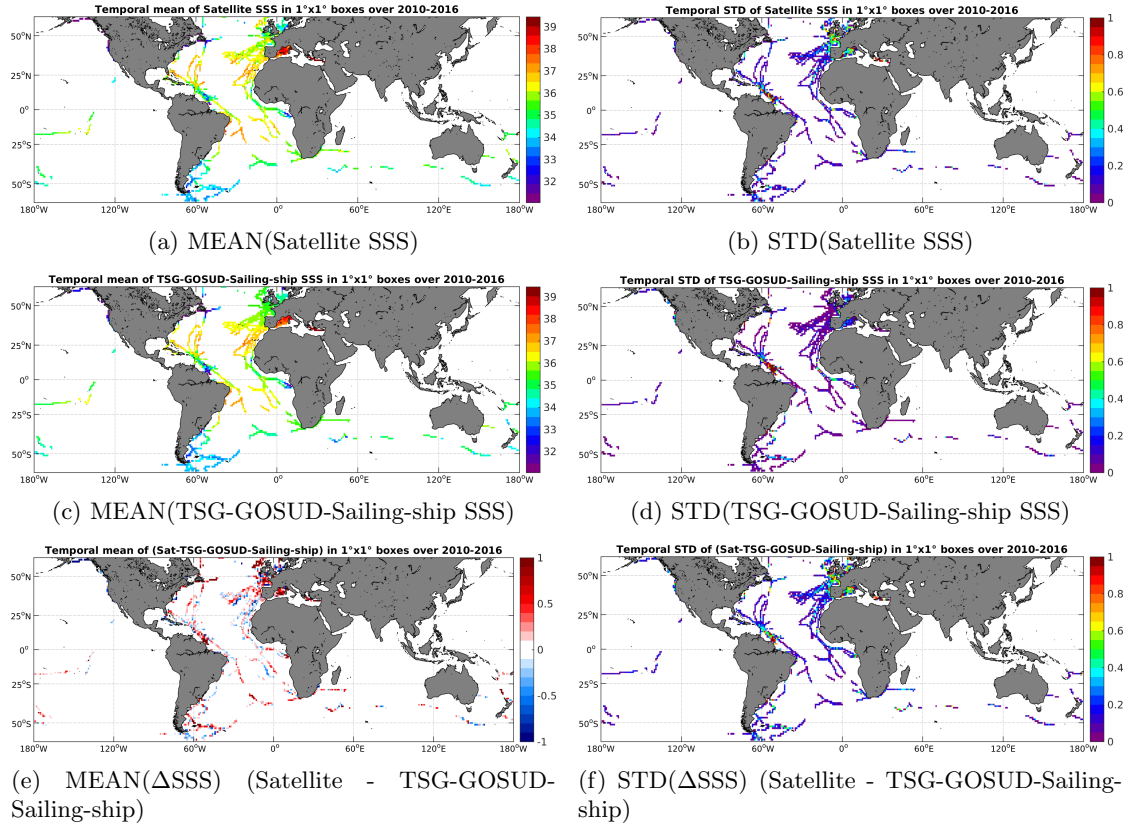
Figure 6: Temporal mean (left) and STD (right) of SSS from SMOS-L3-CATDS-CECOS-LOCEAN-V2-9DAYS-25KM (top), TSG-GOSUD-Sailing-ship (middle), and of \Delta SSS (Satellite - TSG-GOSUD-Sailing-ship). Only match-up pairs are used to generate these maps.
