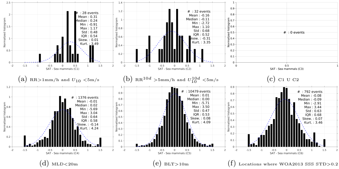
Figure 13: Normalized histogram of \Delta\text{SSS} (SMOS-L3-CATDS-CECOS-LOCEAN-V2-9DAYS-25KM - Sea mammals) for 6 different subdatasets corresponding to: RR > 1mm/h and U_{10} < 5\text{m/s} (a), RR^{10d} > 5\text{mm/h} and U_{10}^{10d} < 5\text{m/s} (b), C1 U C2 (c), MLD < 20m (d), BLT > 10m (e), Locations where WOA2013 SSS STD > 0.2 (f).
