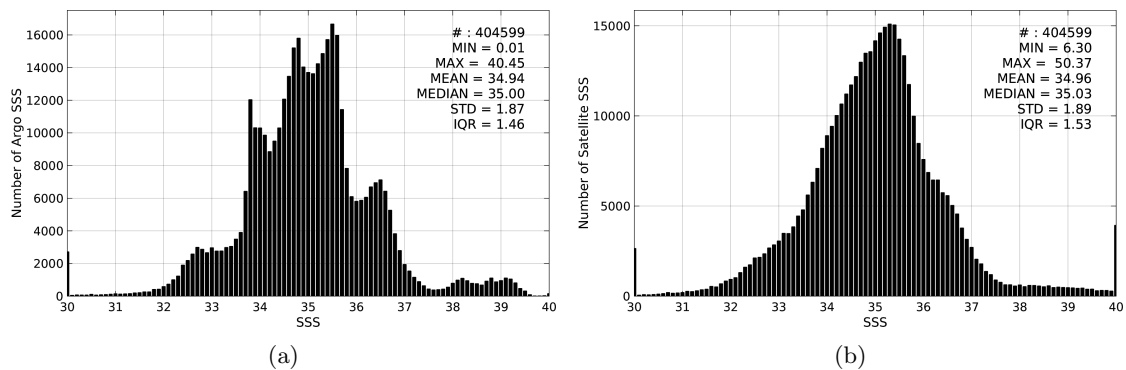
Figure 2: Histograms of SSS from Argo (a) and SMOS-L3-CATDS-CECOS-LOCEAN-V2-9DAYS-25KM (b) considering all match-up pairs per bins of 0.1 over the SMOS coastal zone ( \pm 800 km) 60N-60S Pi-MEP region and for the full satellite product period.
