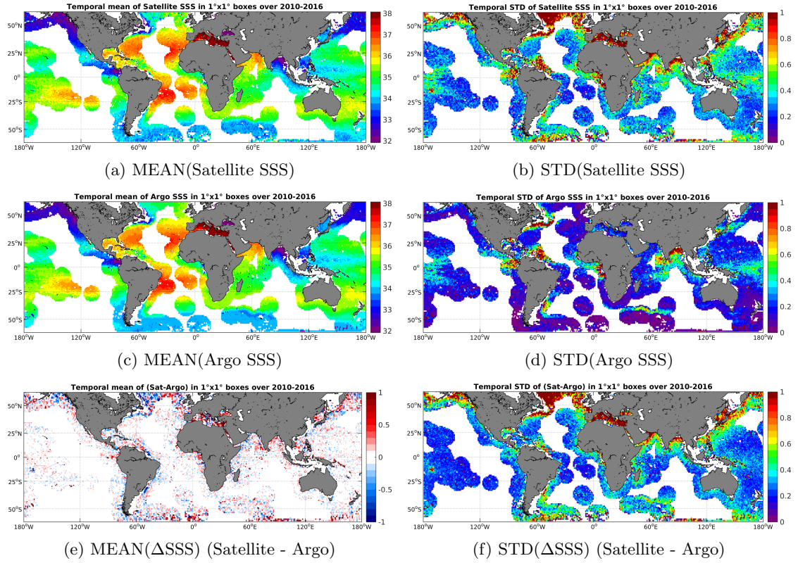
Figure 6: Temporal mean (left) and STD (right) of SSS from SMOS-L3-CATDS-CECOS-LOCEAN-V2-9DAYS-25KM (top), Argo (middle), and of \Delta SSS (Satellite - Argo). Only match-up pairs are used to generate these maps.
