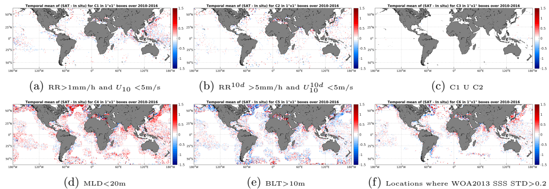
Figure 12: Temporal mean gridded over spatial boxes of size 1^\circ \times 1^\circ of \Delta\text{SSS} (SMOS-L3-CATDS-CECOS-LOCEAN-V2-9DAYS-25KM - Argo) for 6 different subdatasets corresponding to: RR > 1\text{mm/h} and U_{10} < 5\text{m/s} (a), RR^{10d} > 5\text{mm/h} and U_{10}^{10d} < 5\text{m/s} (b), C1 U C2 (c), MLD < 20\text{m} (d), BLT > 10\text{m} (e), Locations where WOA2013 SSS STD > 0.2 (f).
