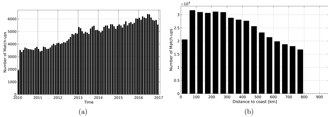
Figure 1: Number of match-ups between Argo and SMOS-L3-CATDS-CECOS-LOCEAN-V2-9DAYS-25KM SSS as a function of time (a) and as function of the distance to coast (b) over the SMOS coastal zone ( \pm 800 km) 60N-60S Pi-MEP region and for the full satellite product period.
