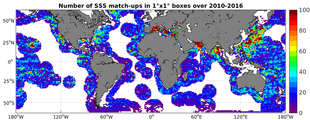
Figure 4: Number of SSS match-ups between Argo SSS and the SMOS-L3-CATDS-CECOS-LOCEAN-V2-9DAYS-25KM SSS product for the SMOS coastal zone ( \pm 800\text{km} ) 60N-60S Pi-MEP region over 1^\circ \times 1^\circ boxes and for the full satellite product period.
