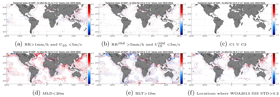
Figure 12: Temporal mean gridded over spatial boxes of size 1^\circ \times 1^\circ of \Delta SSS (SMOS-L3-CATDS-CECOS-LOCEAN-V2-9DAYS-25KM - Argo) for 6 different subdatasets corresponding to: RR > 1\text{mm/h} and U_{10} < 5\text{m/s} (a), RR^{10d} > 5\text{mm/h} and U_{10}^{10d} < 5\text{m/s} (b), C1 U C2 (c), MLD < 20\text{m} (d), BLT > 10\text{m} (e), Locations where WOA2013 SSS STD > 0.2 (f).
