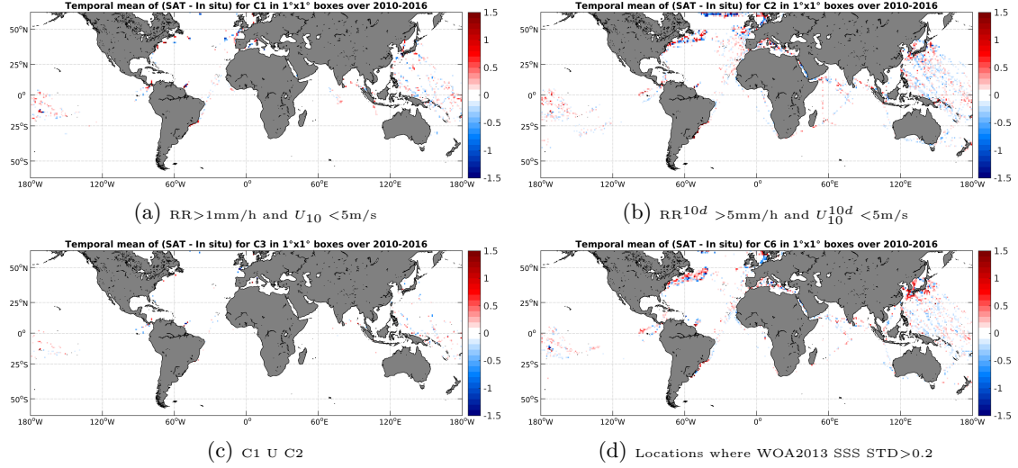
Figure 12: Temporal mean gridded over spatial boxes of size 1^\circ \times 1^\circ of \Delta SSS (SMOS-L3-CATDS-CECOS-LOCEAN-V2-18DAYS-25KM - TSG-LEGOS-DM) for 4 different subdatasets corresponding to: RR > 1mm/h and U_{10} < 5 m/s (a), RR^{10d} > 5 mm/h and U_{10}^{10d} < 5 m/s (b), C1 U C2 (c), Locations where WOA2013 SSS STD > 0.2 (d).
