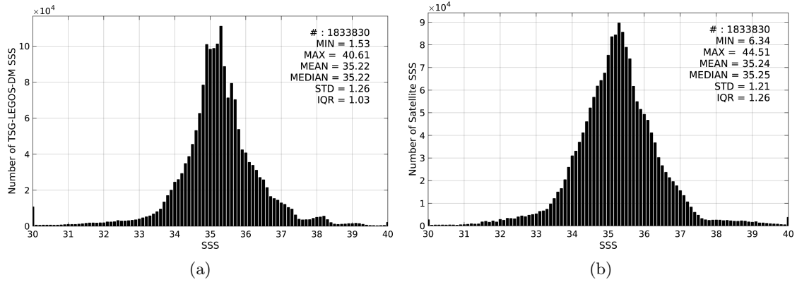
Figure 2: Histograms of SSS from TSG-LEGOS-DM (a) and SMOS-L3-CATDS-CECOS-LOCEAN-V2-18DAYS-25KM (b) considering all match-up pairs per bins of 0.1 over the SMOS coastal zone ( \geq 800 km) 60N-60S Pi-MEP region and for the full satellite product period.
