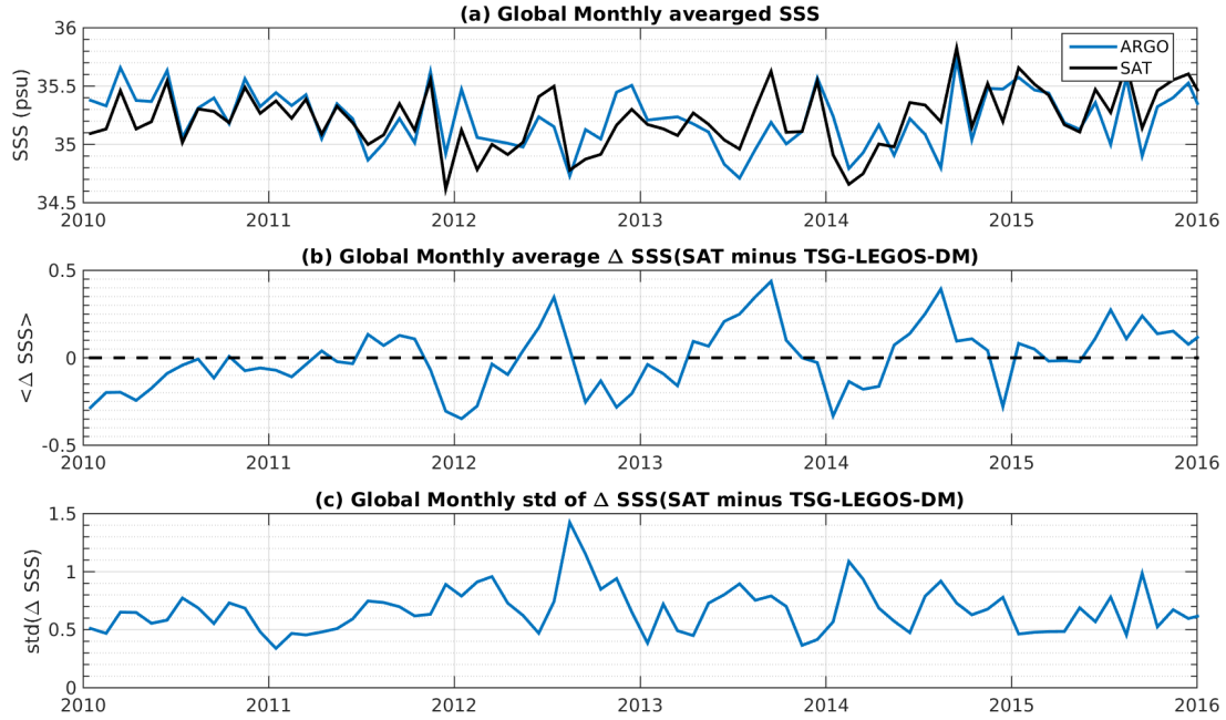
Figure 7: Time series of the monthly averaged mean SSS (top), mean \Delta SSS (Satellite - TSG-LEGOS-DM) and STD of \Delta SSS (Satellite - TSG-LEGOS-DM) over the SMOS coastal zone ( \geq 800\text{km} ) 60N-60S Pi-MEP region considering all match-ups collected by the Pi-MEP platform.
