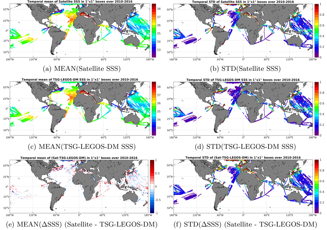
Figure 6: Temporal mean (left) and STD (right) of SSS from SMOS-L3-CATDS-CECOS-LOCEAN-V2-18DAYS-25KM (top), TSG-LEGOS-DM (middle), and of \Delta SSS (Satellite - TSG-LEGOS-DM). Only match-up pairs are used to generate these maps.
