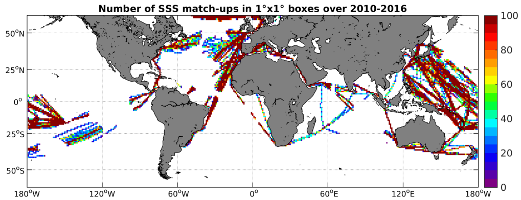
Figure 4: Number of SSS match-ups between TSG-LEGOS-DM SSS and the SMOS-L3-CATDS-CECOS-LOCEAN-V2-18DAYS-25KM SSS product for the SMOS coastal zone ( \geq 800\text{km} ) 60^\circ\text{N} - 60^\circ\text{S} Pi-MEP region over 1^\circ \times 1^\circ boxes and for the full satellite product period.
