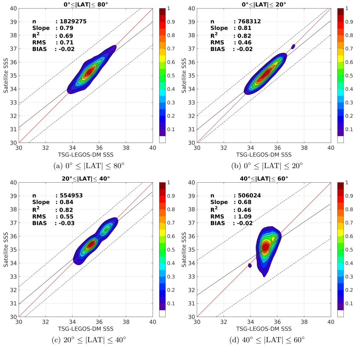
Figure 9: Contour maps of the concentration of SMOS-L3-CATDS-CECOS-LOCEAN-V2-18DAYS-25KM SSS (y-axis) versus TSG-LEGOS-DM SSS (x-axis) at match-up pairs for different latitude bands. For each plot, the red line shows x=y . The black thin and dashed lines indicate a linear fit through the data cloud and the \pm 95\% confidence levels, respectively. The number match-up pairs n , the slope and R^2 coefficient of the linear fit, the root mean square (RMS) and the mean bias between satellite and in situ data are indicated for each latitude band in each plots.
