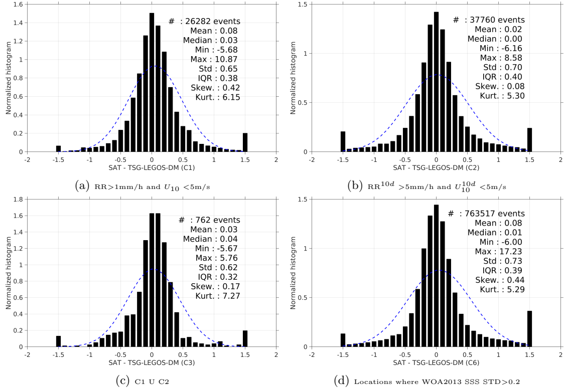
Figure 13: Normalized histogram of \Delta SSS (SMOS-L3-CATDS-CECOS-LOCEAN-V2-18DAYS-25KM - TSG-LEGOS-DM) for 6 different subdatasets corresponding to: RR > 1\text{mm/h} and U_{10} < 5\text{m/s} (a), RR^{10d} > 5\text{mm/h} and U_{10}^{10d} < 5\text{m/s} (b), C1 U C2 (c), Locations where WOA2013 SSS STD > 0.2 (d).
