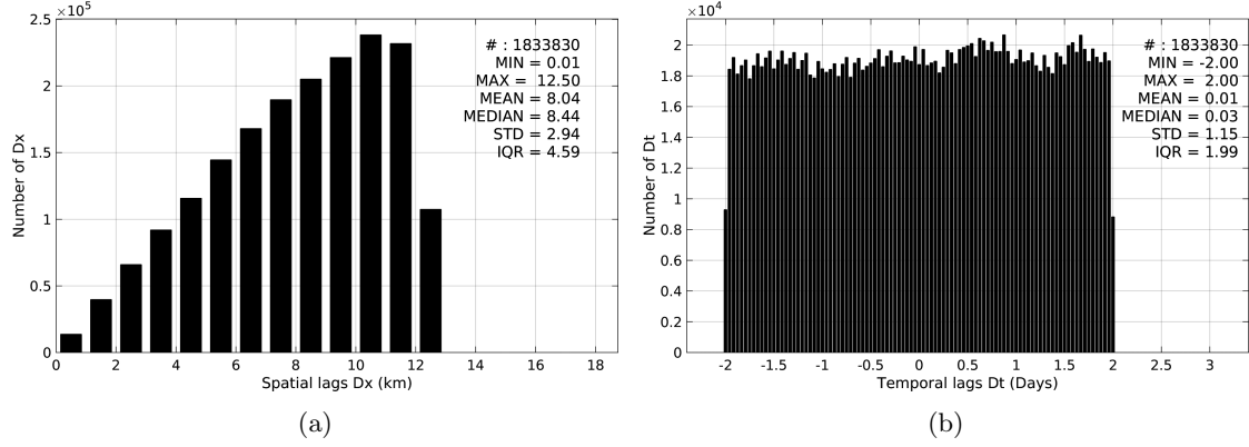
Figure 5: Histograms of the spatial (a) and temporal (b) lags between the time of the TSG-LEGOS-DM measurements and the date of the corresponding SMOS-L3-CATDS-CECOS-LOCEAN-V2-18DAYS-25KM SSS product.
