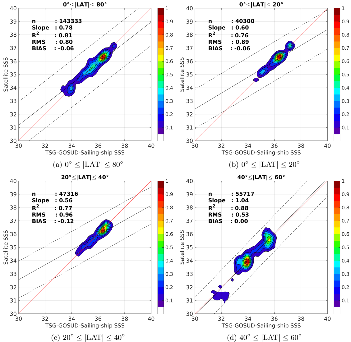
Figure 9: Contour maps of the concentration of SMOS-L3-CATDS-CECOS-LOCEAN-V2-18DAYS-25KM SSS (y-axis) versus TSG-GOSUD-Sailing-ship SSS (x-axis) at match-up pairs for different latitude bands. For each plot, the red line shows x=y . The black thin and dashed lines indicate a linear fit through the data cloud and the \pm 95\% confidence levels, respectively. The number match-up pairs n , the slope and R^2 coefficient of the linear fit, the root mean square (RMS) and the mean bias between satellite and in situ data are indicated for each latitude band in each plots.
