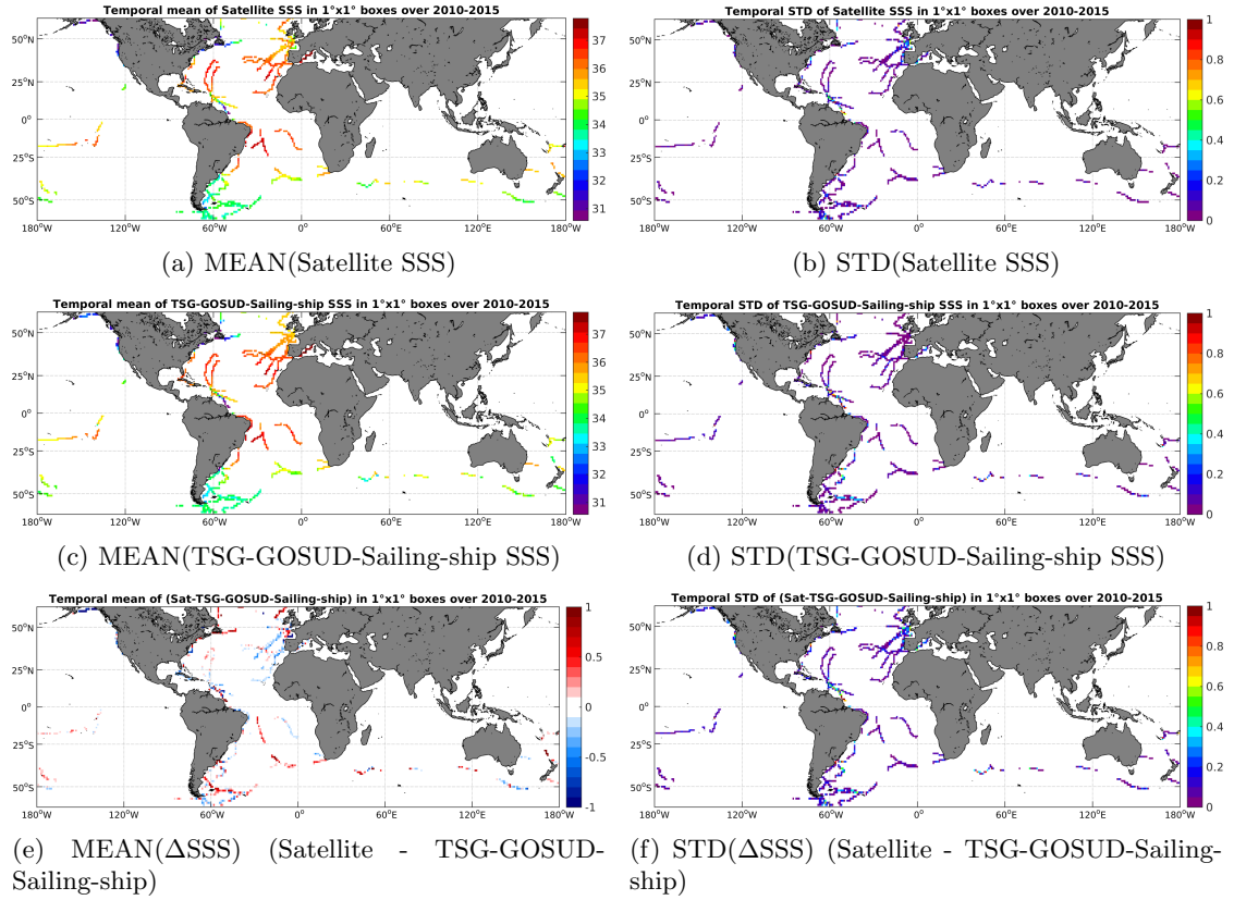
Figure 6: Temporal mean (left) and STD (right) of SSS from SMOS-L3-CATDS-CECOS-LOCEAN-V2-18DAYS-25KM (top), TSG-GOSUD-Sailing-ship (middle), and of \Delta SSS (Satellite - TSG-GOSUD-Sailing-ship). Only match-up pairs are used to generate these maps.
