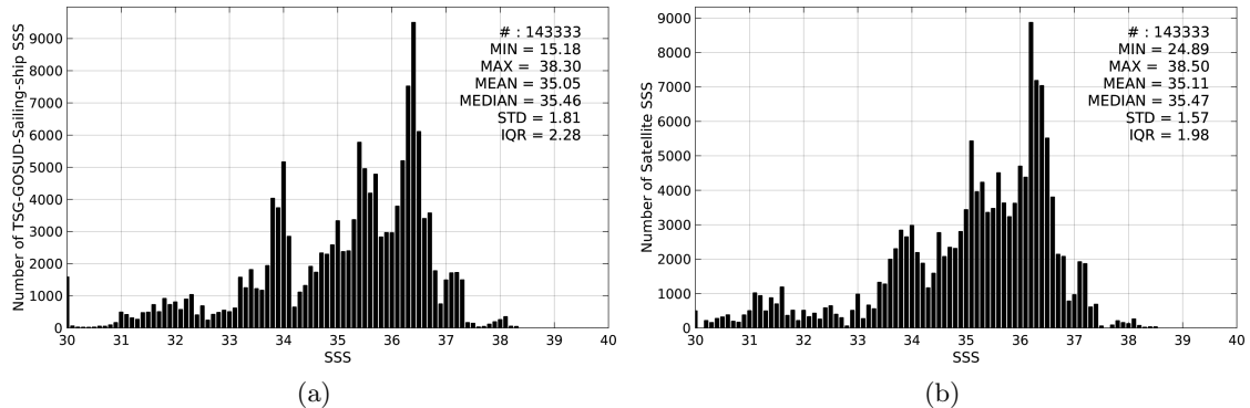
Figure 2: Histograms of SSS from TSG-GOSUD-Sailing-ship (a) and SMOS-L3-CATDS-CECOS-LOCEAN-V2-18DAYS-25KM (b) considering all match-up pairs per bins of 0.1 over the SMOS coastal zone ( \approx 800\text{km} ) 60N-60S Pi-MEP region and for the full satellite product period.
