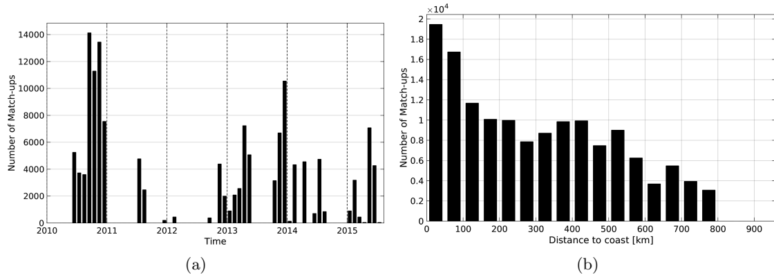
Figure 1: Number of match-ups between TSG-GOSUD-Sailing-ship and SMOS-L3-CATDS-CECOS-LOCEAN-V2-18DAYS-25KM SSS as a function of time (a) and as function of the distance to coast (b) over the SMOS coastal zone ( \approx 800\text{km} ) 60N-60S Pi-MEP region and for the full satellite product period.
