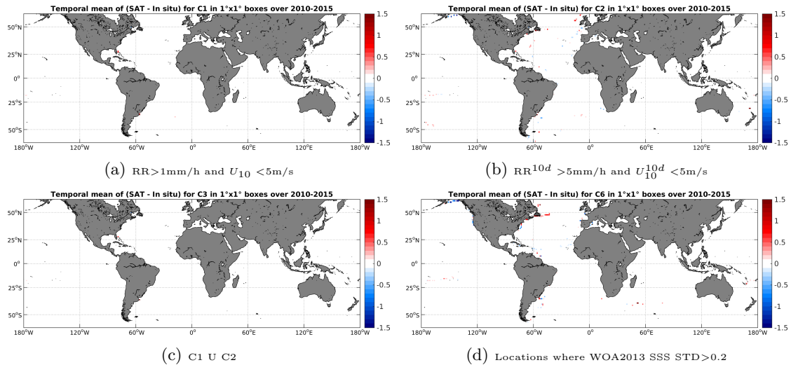
Figure 12: Temporal mean gridded over spatial boxes of size 1^\circ \times 1^\circ of \Delta SSS (SMOS-L3-CATDS-CECOS-LOCEAN-V2-18DAYS-25KM - TSG-GOSUD-Sailing-ship) for 4 different subdatasets corresponding to: RR > 1\text{mm/h} and U_{10} < 5\text{m/s} (a), RR^{10d} > 5\text{mm/h} and U_{10}^{10d} < 5\text{m/s} (b), C1 U C2 (c), Locations where WOA2013 SSS STD > 0.2 (d).
