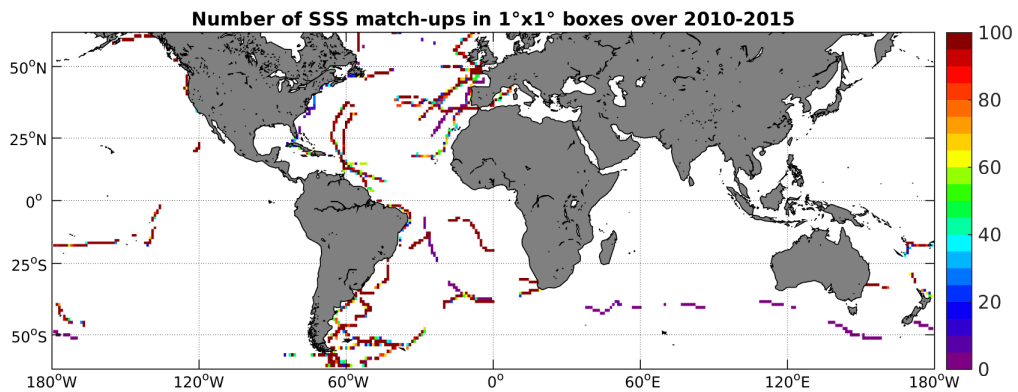
Figure 4: Number of SSS match-ups between TSG-GOSUD-Sailing-ship SSS and the SMOS-L3-CATDS-CECOS-LOCEAN-V2-18DAYS-25KM SSS product for the SMOS coastal zone ( \pm 800\text{km} ) 60N-60S Pi-MEP region over 1^\circ \times 1^\circ boxes and for the full satellite product period.
