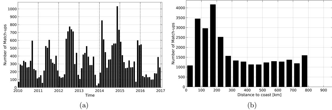
Figure 1: Number of match-ups between Sea mammals and SMOS-L3-CATDS-CECOS-LOCEAN-V2-18DAYS-25KM SSS as a function of time (a) and as function of the distance to coast (b) over the SMOS coastal zone ( \approx 800\text{km} ) 60N-60S Pi-MEP region and for the full satellite product period.
