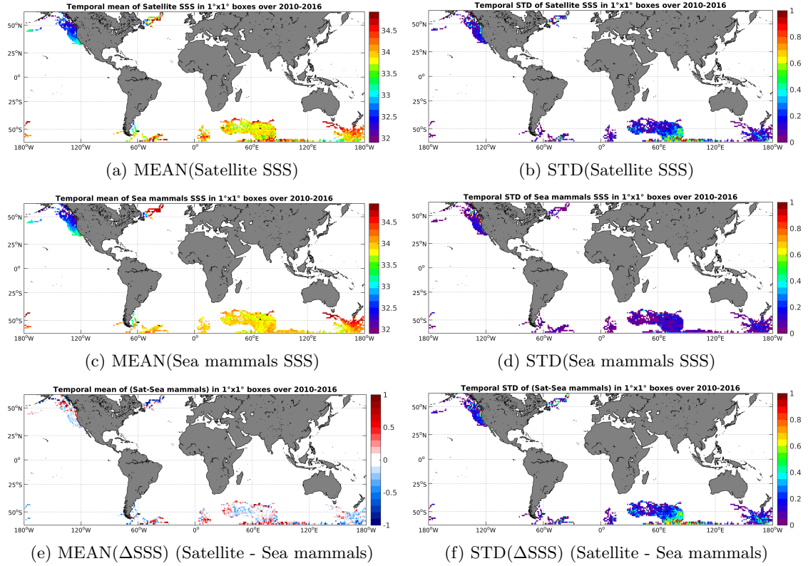
Figure 6: Temporal mean (left) and STD (right) of SSS from SMOS-L3-CATDS-CECOS-LOCEAN-V2-18DAYS-25KM (top), Sea mammals (middle), and of \Delta SSS (Satellite - Sea mammals). Only match-up pairs are used to generate these maps.
