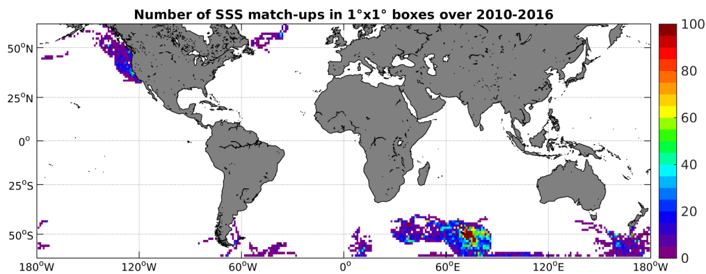
Figure 4: Number of SSS match-ups between Sea mammals SSS and the SMOS-L3-CATDS-CECOS-LOCEAN-V2-18DAYS-25KM SSS product for the SMOS coastal zone ( \approx 800\text{km} ) 60N-60S Pi-MEP region over 1^\circ \times 1^\circ boxes and for the full satellite product period.
