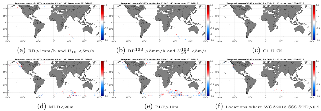
Figure 12: Temporal mean gridded over spatial boxes of size 1^\circ \times 1^\circ of \Delta SSS (SMOS-L3-CATDS-CECOS-LOCEAN-V2-18DAYS-25KM - Sea mammals) for 6 different subdatasets corresponding to: RR > 1\text{mm/h} and U_{10} < 5\text{m/s} (a), RR^{10d} > 5\text{mm/h} and U_{10}^{10d} < 5\text{m/s} (b), C1 U C2 (c), MLD < 20\text{m} (d), BLT > 10\text{m} (e), Locations where WOA2013 SSS STD > 0.2 (f).
