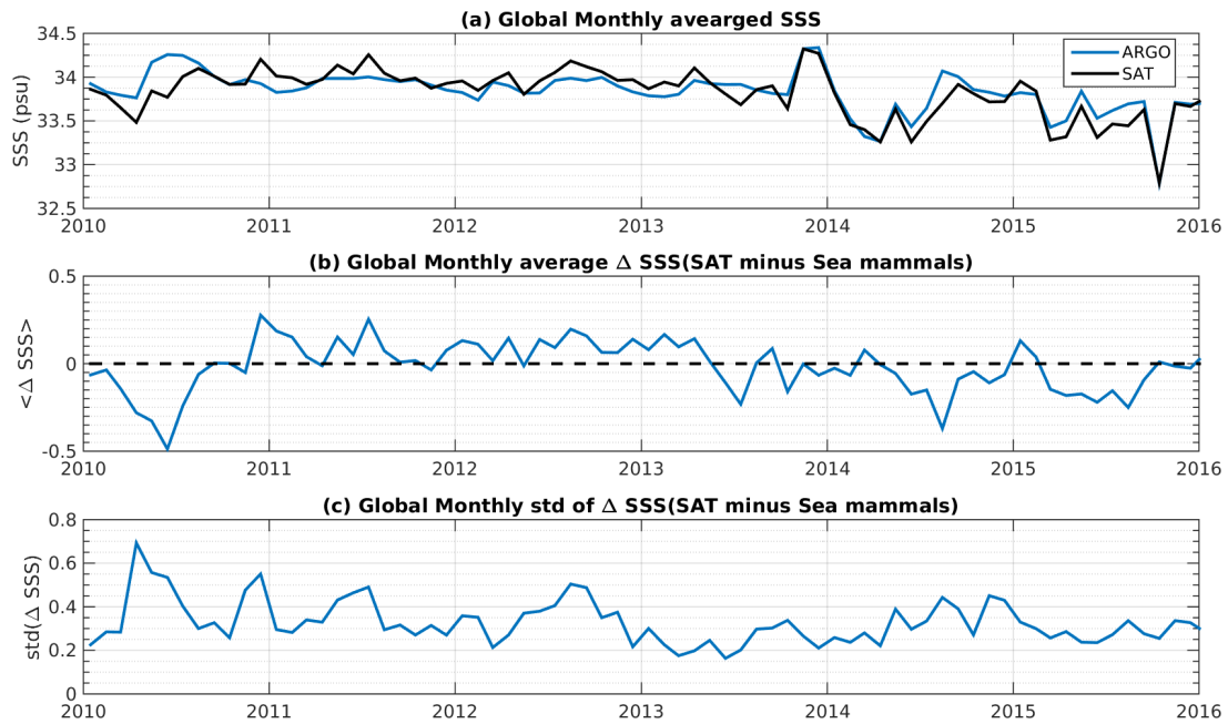
Figure 7: Time series of the monthly averaged mean SSS (top), mean \Delta SSS (Satellite - Sea mammals) and STD of \Delta SSS (Satellite - Sea mammals) over the SMOS coastal zone ( \pm 800 km) 60N-60S Pi-MEP region considering all match-ups collected by the Pi-MEP platform.
