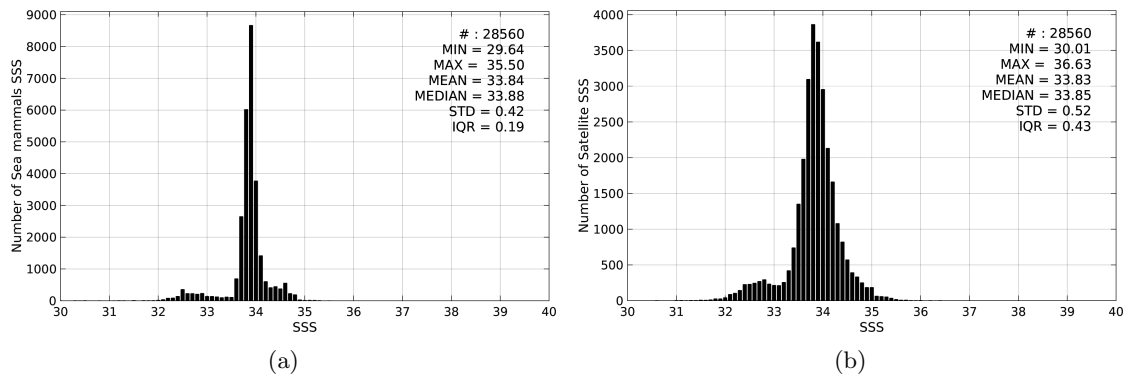
Figure 2: Histograms of SSS from Sea mammals (a) and SMOS-L3-CATDS-CECOS-LOCEAN-V2-18DAYS-25KM (b) considering all match-up pairs per bins of 0.1 over the SMOS coastal zone ( \approx 800\text{km} ) 60N-60S Pi-MEP region and for the full satellite product period.
