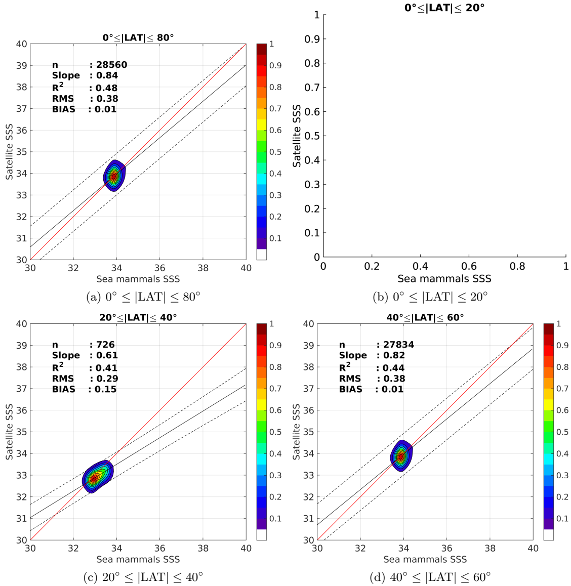
Figure 9: Contour maps of the concentration of SMOS-L3-CATDS-CECOS-LOCEAN-V2-18DAYS-25KM SSS (y-axis) versus Sea mammals SSS (x-axis) at match-up pairs for different latitude bands. For each plot, the red line shows x=y . The black thin and dashed lines indicate a linear fit through the data cloud and the \pm 95\% confidence levels, respectively. The number match-up pairs n , the slope and R^2 coefficient of the linear fit, the root mean square (RMS) and the mean bias between satellite and in situ data are indicated for each latitude band in each plots.
