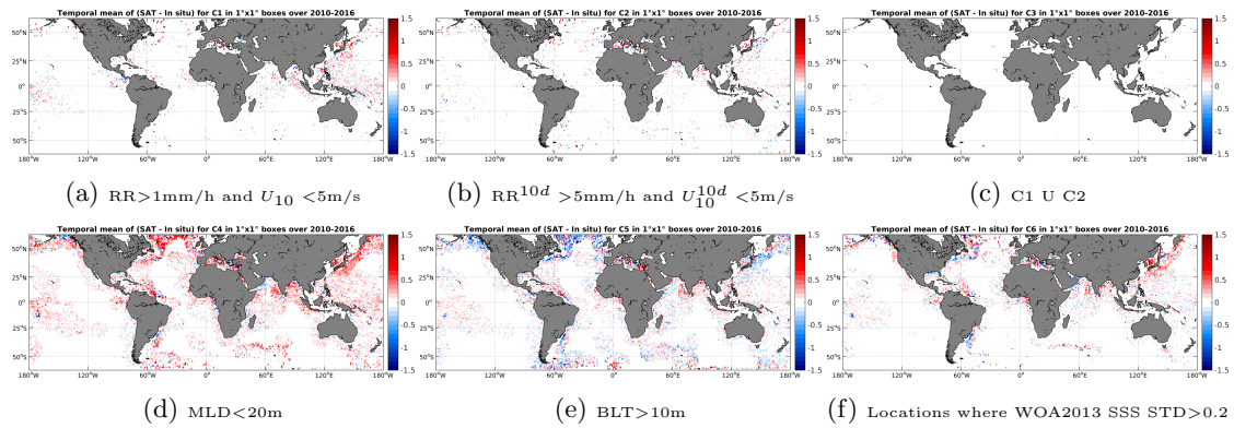
Figure 12: Temporal mean gridded over spatial boxes of size 1^\circ \times 1^\circ of \Delta SSS (SMOS-L3-CATDS-CECOS-LOCEAN-V2-18DAYS-25KM - Argo) for 6 different subdatasets corresponding to: RR > 1\text{mm/h} and U_{10} < 5\text{m/s} (a), RR^{10d} > 5\text{mm/h} and U_{10}^{10d} < 5\text{m/s} (b), C1 U C2 (c), MLD < 20\text{m} (d), BLT > 10\text{m} (e), Locations where WOA2013 SSS STD > 0.2 (f).
