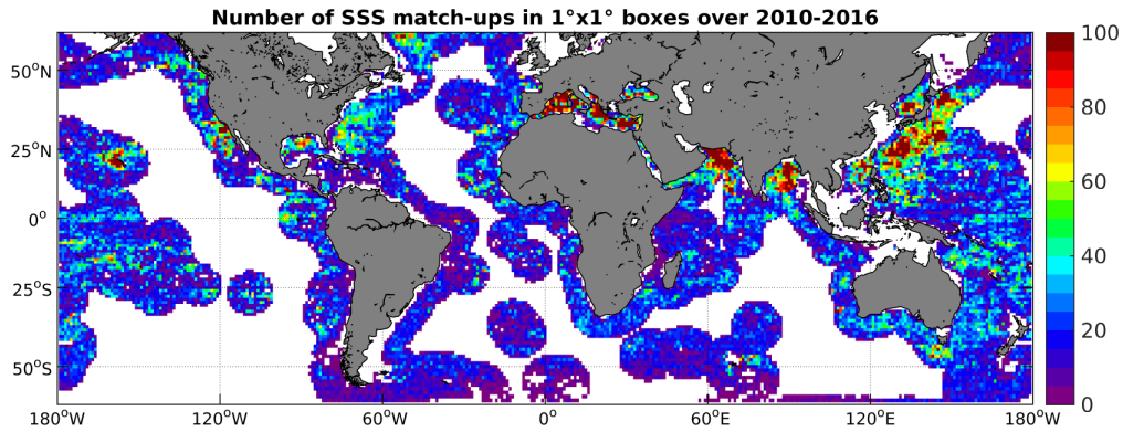
Figure 4: Number of SSS match-ups between Argo SSS and the SMOS-L3-CATDS-CECOS-LOCEAN-V2-18DAYS-25KM SSS product for the SMOS coastal zone ( \pm 800\text{km} ) 60N-60S Pi-MEP region over 1^\circ \times 1^\circ boxes and for the full satellite product period.
