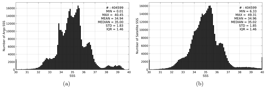
Figure 2: Histograms of SSS from Argo (a) and SMOS-L3-CATDS-CECOS-LOCEAN-V2-18DAYS-25KM (b) considering all match-up pairs per bins of 0.1 over the SMOS coastal zone ( \pm 800 km) 60N-60S Pi-MEP region and for the full satellite product period.
