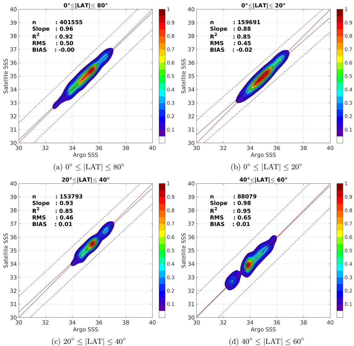
Figure 9: Contour maps of the concentration of SMOS-L3-CATDS-CECOS-LOCEAN-V2-18DAYS-25KM SSS (y-axis) versus Argo SSS (x-axis) at match-up pairs for different latitude bands. For each plot, the red line shows x=y . The black thin and dashed lines indicate a linear fit through the data cloud and the \pm 95\% confidence levels, respectively. The number match-up pairs n , the slope and R^2 coefficient of the linear fit, the root mean square (RMS) and the mean bias between satellite and in situ data are indicated for each latitude band in each plots.
