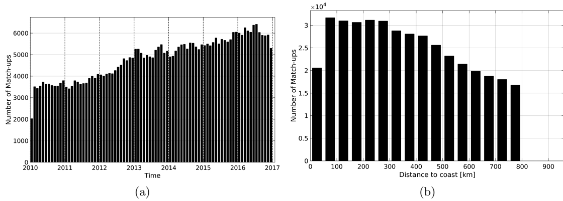
Figure 1: Number of match-ups between Argo and SMOS-L3-CATDS-CECOS-LOCEAN-V2-18DAYS-25KM SSS as a function of time (a) and as function of the distance to coast (b) over the SMOS coastal zone ( \pm 800 km) 60N-60S Pi-MEP region and for the full satellite product period.
