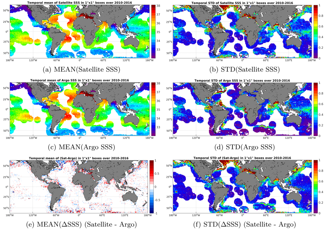
Figure 6: Temporal mean (left) and STD (right) of SSS from SMOS-L3-CATDS-CECOS-LOCEAN-V2-18DAYS-25KM (top), Argo (middle), and of \Delta SSS (Satellite - Argo). Only match-up pairs are used to generate these maps.
