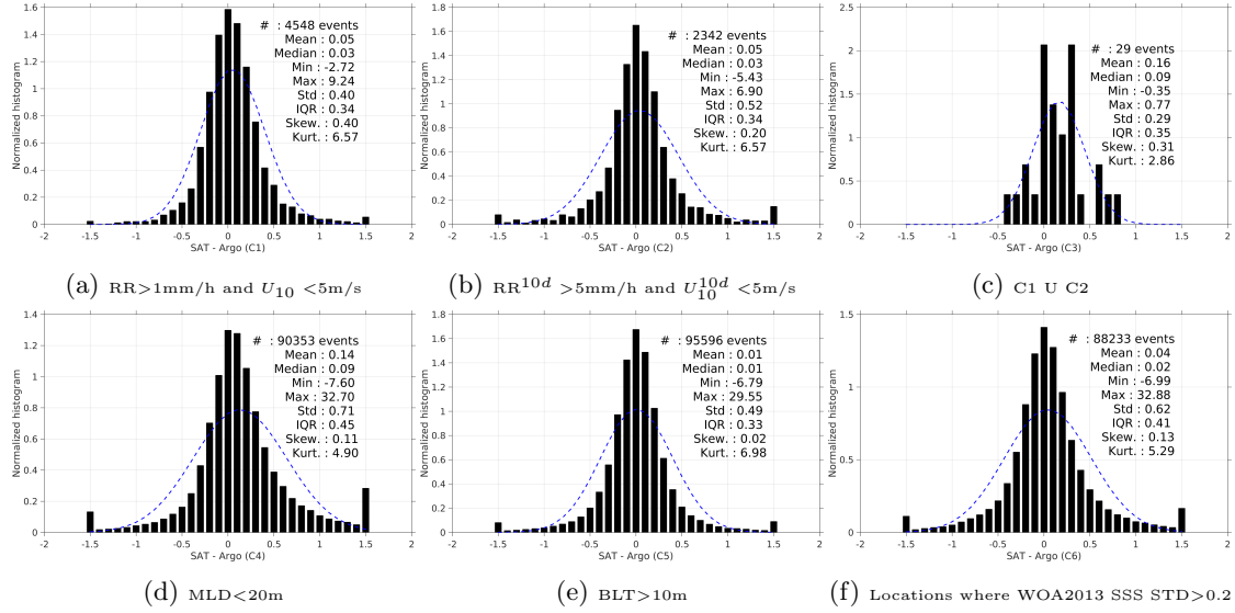
Figure 13: Normalized histogram of \Delta SSS (SMOS-L3-CATDS-CECOS-LOCEAN-V2-18DAYS-25KM - Argo) for 6 different subdatasets corresponding to: RR>1mm/h and U_{10} <5m/s (a), RR 10d >5mm/h and U_{10}^{10d} <5m/s (b), C1 U C2 (c),MLD<20m (d),BLT>10m (e),Locations where WOA2013 SSS STD>0.2 (f).
