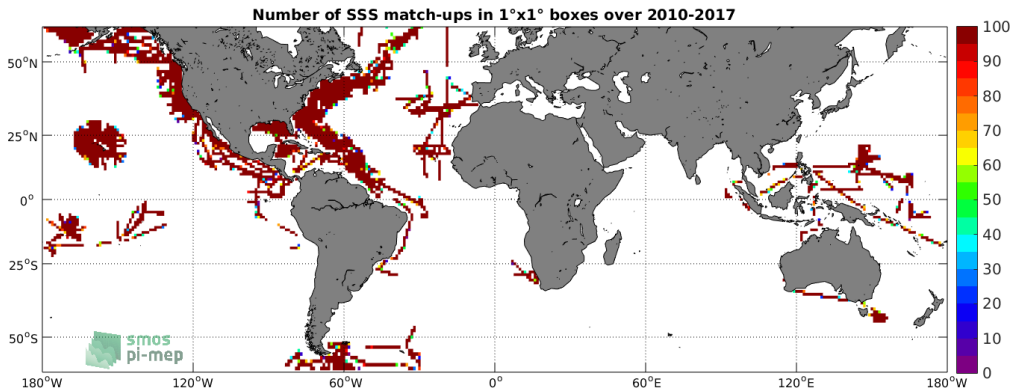
Figure 4: Number of SSS match-ups between TSG (SAMOS) SSS and the SMOS SSS L3 v2 - Monthly - 0.25 Deg (CATDS-CECOS-IFREMER) SSS product for the SMOS coastal zone (<800km) 60N-60S Pi-MEP region over 1^\circ \times 1^\circ boxes and for the full satellite product period.
