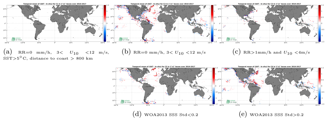
Figure 12: Temporal mean gridded over spatial boxes of size 1^\circ \times 1^\circ of \Delta SSS (SMOS SSS L3 v2 - Monthly - 0.25 Deg (CATDS-CECOS-IFREMER) - TSG (SAMOS)) for 5 different subdatasets corresponding to: RR=0 mm/h, 3 < U_{10} < 12 m/s, SST > 5^\circ\text{C} , distance to coast > 800 km (a), RR=0 mm/h, 3 < U_{10} < 12 m/s (b), RR > 1 mm/h and U_{10} < 4 m/s (c), WOA2013 SSS Std < 0.2 (d), WOA2013 SSS Std > 0.2 (e).
