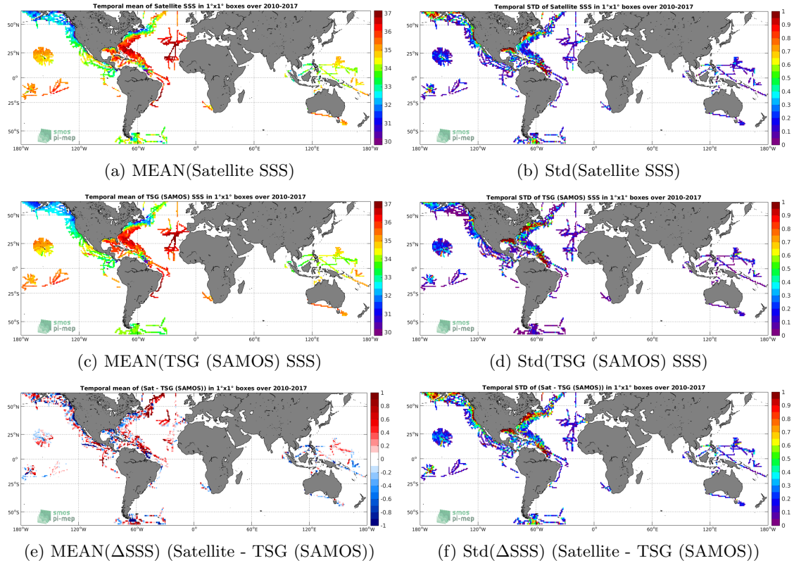
Figure 6: Temporal mean (left) and Std (right) of SSS from SMOS SSS L3 v2 - Monthly - 0.25 Deg (CATDS-CECOS-IFREMER) (top), TSG (SAMOS) (middle), and of \Delta SSS (Satellite - TSG (SAMOS)). Only match-up pairs are used to generate these maps.
