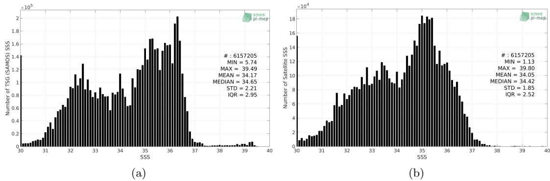
Figure 2: Histograms of SSS from TSG (SAMOS) (a) and SMOS SSS L3 v2 - Monthly - 0.25 Deg (CATDS-CECOS-IFREMER) (b) considering all match-up pairs per bins of 0.1 over the SMOS coastal zone (<800km) 60N-60S Pi-MEP region and for the full satellite product period.
