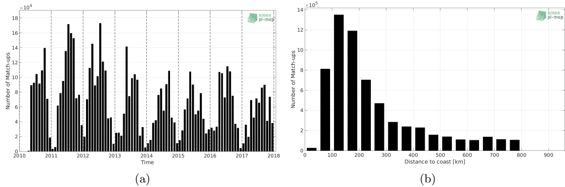
Figure 1: Number of match-ups between TSG (SAMOS) and SMOS SSS L3 v2 - Monthly - 0.25 Deg (CATDS-CECOS-IFREMER) SSS as a function of time (a) and as function of the distance to coast (b) over the SMOS coastal zone (<800km) 60N-60S Pi-MEP region and for the full satellite product period.
