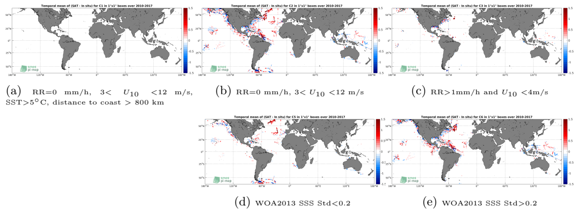
Figure 12: Temporal mean gridded over spatial boxes of size 1^\circ \times 1^\circ of \Delta SSS (SMOS L3 v2 - Monthly - 0.25 Deg (CATDS-CECOS-IFREMER) - TSG-SAMOS) for 5 different subdatasets corresponding to:RR=0 mm/h, 3 < U_{10} < 12 m/s, SST >5^\circ\text{C} , distance to coast > 800 km (a), RR=0 mm/h, 3 < U_{10} < 12 m/s (b), RR >1 mm/h and U_{10} < 4 m/s (c), WOA2013 SSS Std <0.2 (d), WOA2013 SSS Std >0.2 (e).
