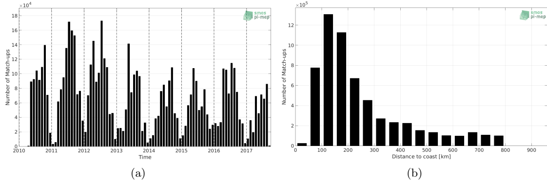
Figure 1: Number of match-ups between TSG-SAMOS and SMOS L3 v2 - Monthly - 0.25 Deg (CATDS-CECOS-IFREMER) SSS as a function of time (a) and as function of the distance to coast (b) over the SMOS coastal zone (<800km) 60N-60S Pi-MEP region and for the full satellite product period.
