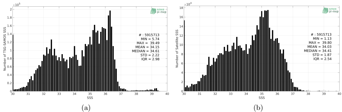
Figure 2: Histograms of SSS from TSG-SAMOS (a) and SMOS L3 v2 - Monthly - 0.25 Deg (CATDS-CECOS-IFREMER) (b) considering all match-up pairs per bins of 0.1 over the SMOS coastal zone (<800km) 60N-60S Pi-MEP region and for the full satellite product period.
