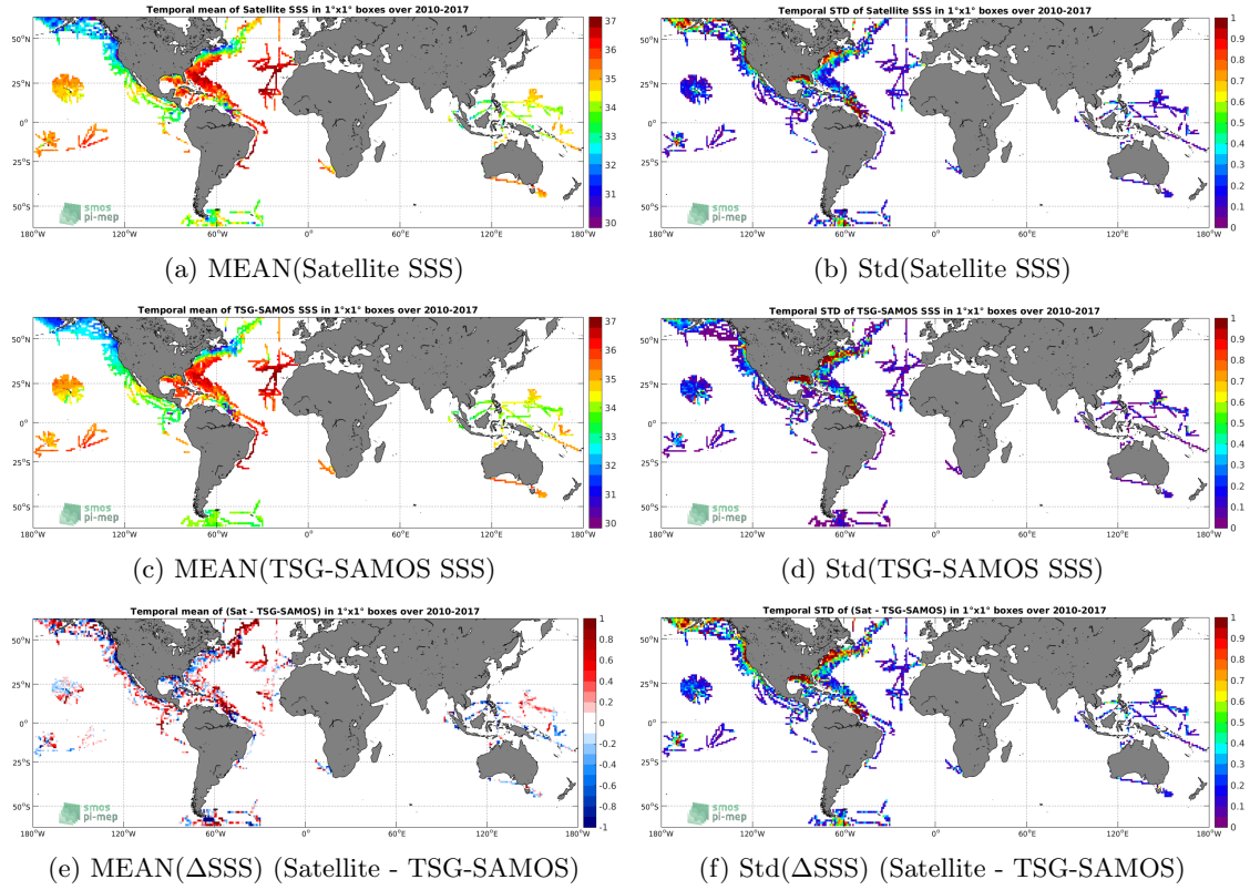
Figure 6: Temporal mean (left) and Std (right) of SSS from SMOS L3 v2 - Monthly - 0.25 Deg (CATDS-CECOS-IFREMER) (top), TSG-SAMOS (middle), and of \Delta SSS (Satellite - TSG-SAMOS). Only match-up pairs are used to generate these maps.
