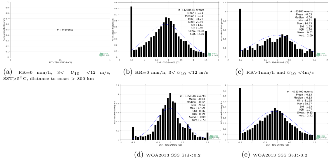
Figure 13: Normalized histogram of \Delta SSS (SMOS L3 v2 - Monthly - 0.25 Deg (CATDS-CECOS-IFREMER) - TSG-SAMOS) for 5 different subdatasets corresponding to: RR=0 mm/h, 3 < U_{10} < 12 m/s, SST > 5°C, distance to coast > 800 km (a), RR=0 mm/h, 3 < U_{10} < 12 m/s (b), RR > 1mm/h and U_{10} < 4 m/s (c), WOA2013 SSS Std < 0.2 (d), WOA2013 SSS Std > 0.2 (e).
