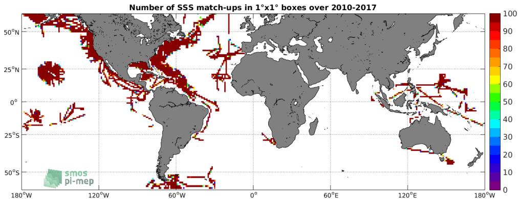
Figure 4: Number of SSS match-ups between TSG-SAMOS SSS and the SMOS L3 v2 - Monthly - 0.25 Deg (CATDS-CECOS-IFREMER) SSS product for the SMOS coastal zone (<800km) 60N-60S Pi-MEP region over 1°x1° boxes and for the full satellite product period.
