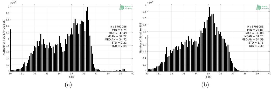
Figure 2: Histograms of SSS from TSG-SAMOS (a) and SMOS-L3-CATDS-IFREMER-CECOS-V2-MONTHLY-0.25DEG (b) considering all match-up pairs per bins of 0.1 over the SMOS coastal zone ( \approx 800 km) 60N-60S Pi-MEP region and for the full satellite product period.
