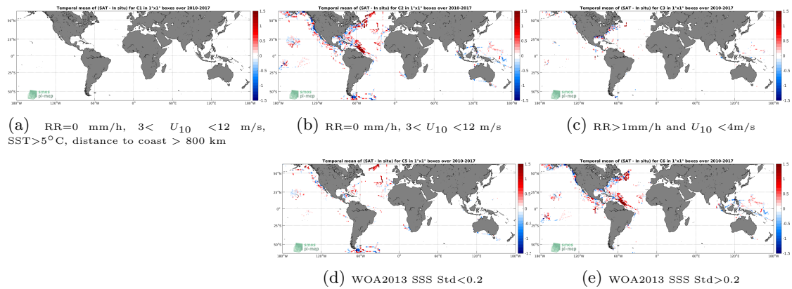
Figure 12: Temporal mean gridded over spatial boxes of size 1^\circ \times 1^\circ of \Delta SSS (SMOS-L3-CATDS-IFREMER-CECOS-V2-MONTHLY-0.25DEG - TSG-SAMOS) for 5 different subdatasets corresponding to:RR=0 mm/h, 3 < U_{10} < 12 m/s, SST >5^\circ C, distance to coast > 800 km (a), RR=0 mm/h, 3 < U_{10} < 12 m/s (b), RR >1 mm/h and U_{10} < 4 m/s (c), WOA2013 SSS Std <0.2 (d), WOA2013 SSS Std >0.2 (e).
