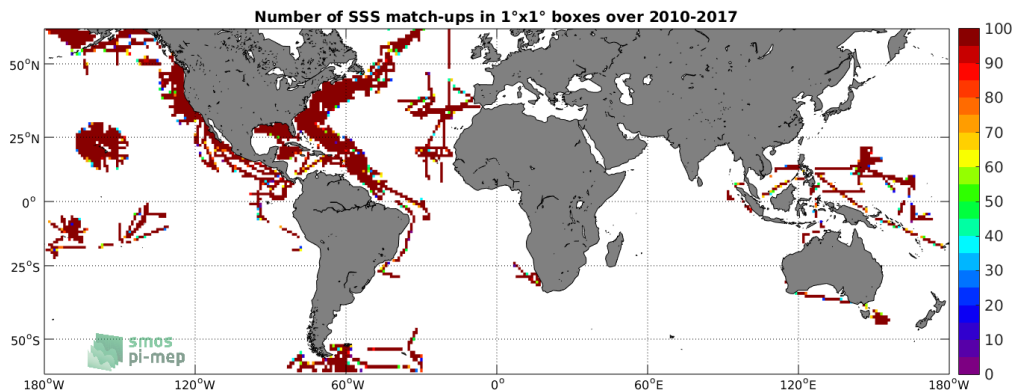
Figure 4: Number of SSS match-ups between TSG-SAMOS SSS and the SMOS-L3-CATDS-IFREMER-CECOS-V2-MONTHLY-0.25DEG SSS product for the SMOS coastal zone ( \approx 800\text{km} ) 60N-60S Pi-MEP region over 1^\circ \times 1^\circ boxes and for the full satellite product period.
