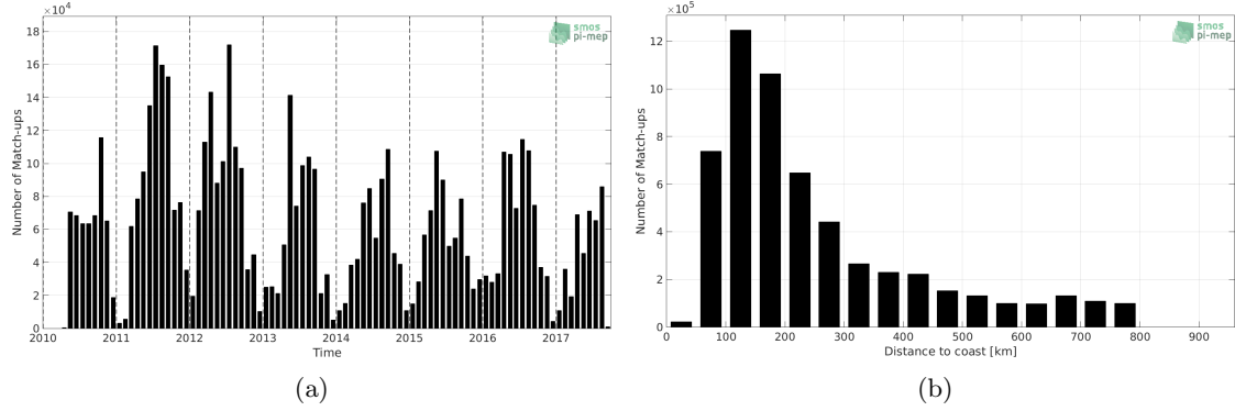
Figure 1: Number of match-ups between TSG-SAMOS and SMOS-L3-CATDS-IFREMER-CECOS-V2-MONTHLY-0.25DEG SSS as a function of time (a) and as function of the distance to coast (b) over the SMOS coastal zone ( \approx 800 km) 60N-60S Pi-MEP region and for the full satellite product period.
