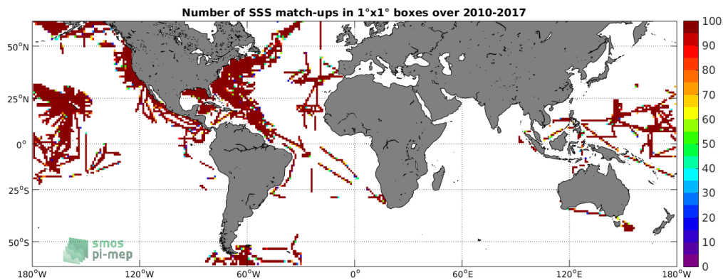
Figure 4: Number of SSS match-ups between TSG-SAMOS SSS and the SMOS-L3-CATDS-IFREMER-CECOS-V2-MONTHLY-0.25DEG SSS product for the SMOS coastal zone ( \pm 800 km) 60N-60S Pi-MEP region over 1^\circ \times 1^\circ boxes and for the full satellite product period.
