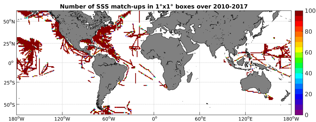
Figure 4: Number of SSS match-ups between TSG-SAMOS SSS and the SMOS-L3-CATDS-IFREMER-CECOS-V2-MONTHLY-0.25DEG SSS product for the SMOS coastal zone ( \approx 800 km) 60N-60S Pi-MEP region over 1^\circ \times 1^\circ boxes and for the full satellite product period.
