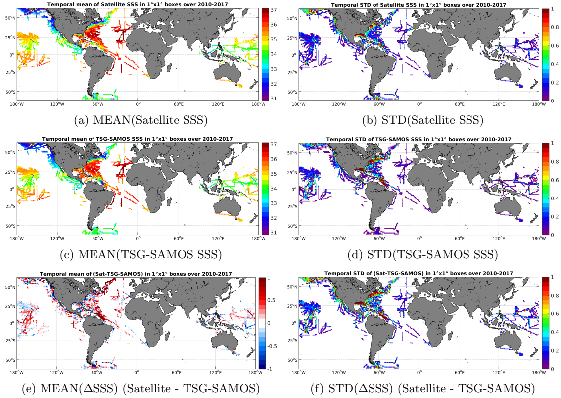
Figure 6: Temporal mean (left) and STD (right) of SSS from SMOS-L3-CATDS-IFREMER-CECOS-V2-MONTHLY-0.25DEG (top), TSG-SAMOS (middle), and of \Delta SSS (Satellite - TSG-SAMOS). Only match-up pairs are used to generate these maps.
