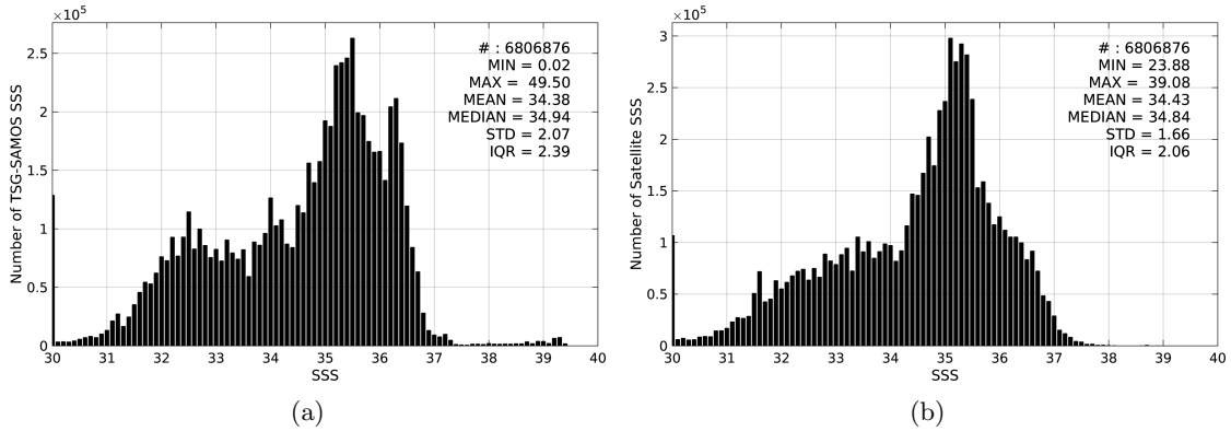
Figure 2: Histograms of SSS from TSG-SAMOS (a) and SMOS-L3-CATDS-IFREMER-CECOS-V2-MONTHLY-0.25DEG (b) considering all match-up pairs per bins of 0.1 over the SMOS coastal zone ( \geq 800 km) 60N-60S Pi-MEP region and for the full satellite product period.
