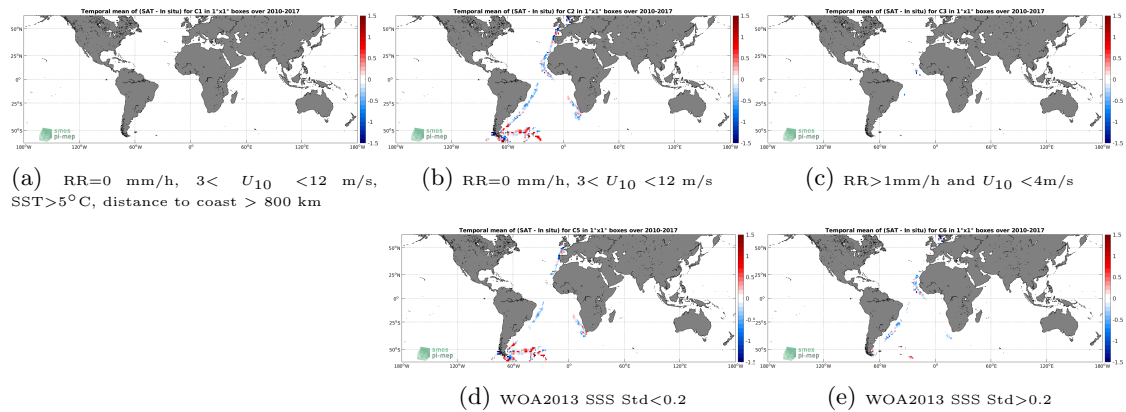
Figure 12: Temporal mean gridded over spatial boxes of size 1^\circ \times 1^\circ of \Delta\text{SSS} (SMOS SSS L3 v2 - Monthly - 0.25 Deg (CATDS-CECOS-IFREMER) - TSG (Polarstern)) for 5 different subdatasets corresponding to: RR=0 mm/h, 3 < U_{10} < 12 m/s, SST >5^\circ\text{C} , distance to coast > 800 km (a), RR=0 mm/h, 3 < U_{10} < 12 m/s (b), RR >1 mm/h and U_{10} < 4 m/s (c), WOA2013 SSS Std <0.2 (d), WOA2013 SSS Std >0.2 (e).
