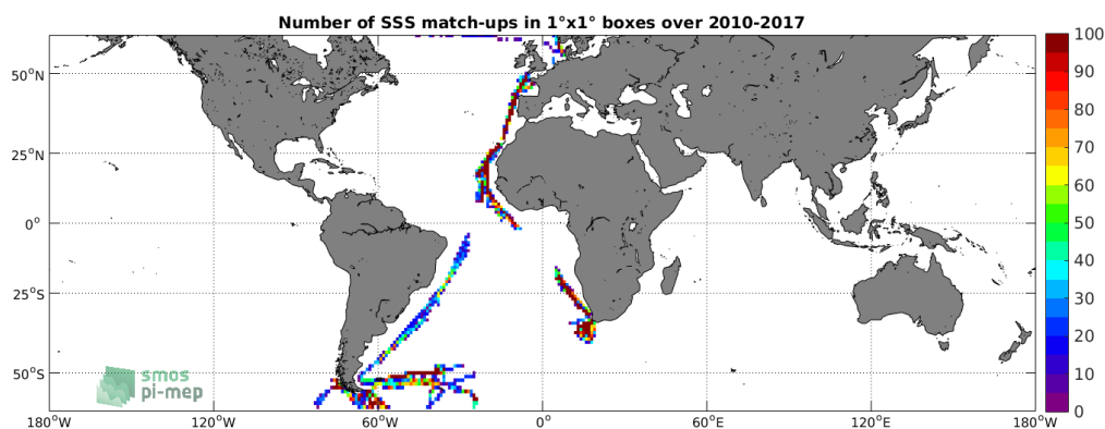
Figure 4: Number of SSS match-ups between TSG-POLARSTERN SSS and the SMOS L3 v2 - Monthly - 0.25 Deg (CATDS-CECOS-IFREMER) SSS product for the SMOS coastal zone (<800km) 60N-60S Pi-MEP region over 1^\circ \times 1^\circ boxes and for the full satellite product period.
