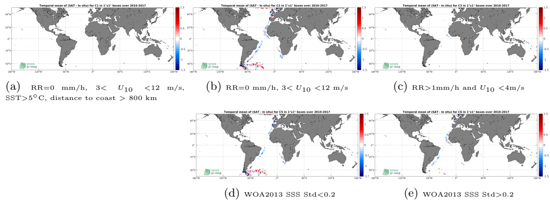
Figure 12: Temporal mean gridded over spatial boxes of size 1^\circ \times 1^\circ of \Delta SSS (SMOS L3 v2 - Monthly - 0.25 Deg (CATDS-CECOS-IFREMER) - TSG-POLARSTERN) for 5 different sub-datasets corresponding to: RR=0 mm/h, 3 < U_{10} < 12 m/s, SST >5^\circ C, distance to coast > 800 km (a), RR=0 mm/h, 3 < U_{10} < 12 m/s (b), RR >1 mm/h and U_{10} < 4 m/s (c), WOA2013 SSS Std <0.2 (d), WOA2013 SSS Std >0.2 (e).
