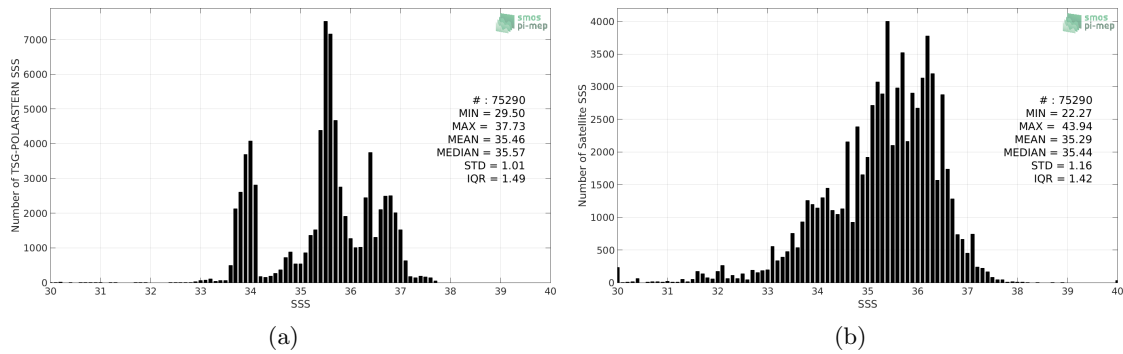
Figure 2: Histograms of SSS from TSG-POLARSTERN (a) and SMOS L3 v2 - Monthly - 0.25 Deg (CATDS-CECOS-IFREMER) (b) considering all match-up pairs per bins of 0.1 over the SMOS coastal zone (<800km) 60N-60S Pi-MEP region and for the full satellite product period.
