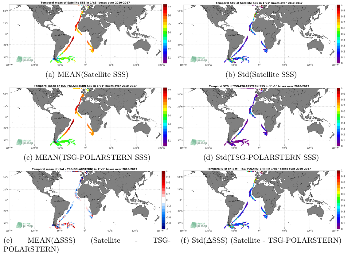
Figure 6: Temporal mean (left) and Std (right) of SSS from SMOS L3 v2 - Monthly - 0.25 Deg (CATDS-CECOS-IFREMER) (top), TSG-POLARSTERN (middle), and of \Delta SSS (Satellite - TSG-POLARSTERN). Only match-up pairs are used to generate these maps.
