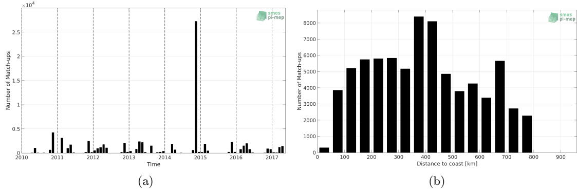
Figure 1: Number of match-ups between TSG-POLARSTERN and SMOS L3 v2 - Monthly - 0.25 Deg (CATDS-CECOS-IFREMER) SSS as a function of time (a) and as function of the distance to coast (b) over the SMOS coastal zone (<800km) 60N-60S Pi-MEP region and for the full satellite product period.
