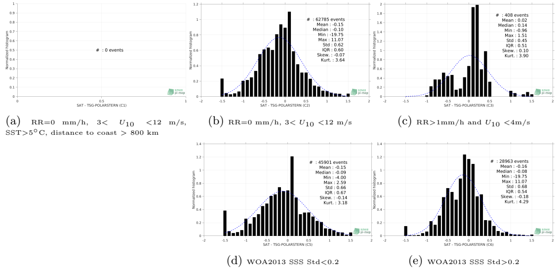
Figure 13: Normalized histogram of \Delta SSS (SMOS-L3-CATDS-IFREMER-CECOS-V2-MONTHLY-0.25DEG - TSG-POLARSTERN) for 5 different subdatasets corresponding to: RR=0 mm/h, 3 < U_{10} < 12 m/s, SST > 5°C, distance to coast > 800 km (a), RR=0 mm/h, 3 < U_{10} < 12 m/s (b), RR > 1mm/h and U_{10} < 4 m/s (c), WOA2013 SSS Std < 0.2 (d), WOA2013 SSS Std > 0.2 (e).
