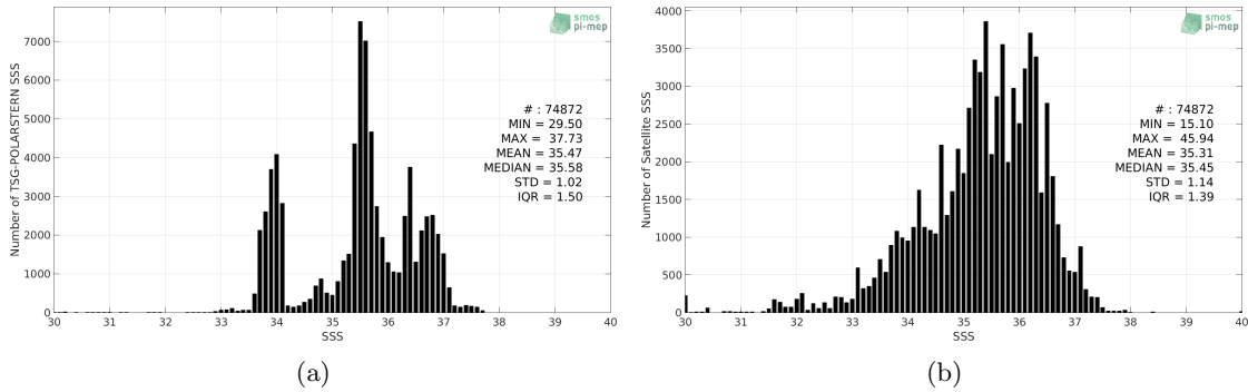
Figure 2: Histograms of SSS from TSG-POLARSTERN (a) and SMOS-L3-CATDS-IFREMER-CECOS-V2-MONTHLY-0.25DEG (b) considering all match-up pairs per bins of 0.1 over the SMOS coastal zone ( \geq 800\text{km} ) 60N-60S Pi-MEP region and for the full satellite product period.
