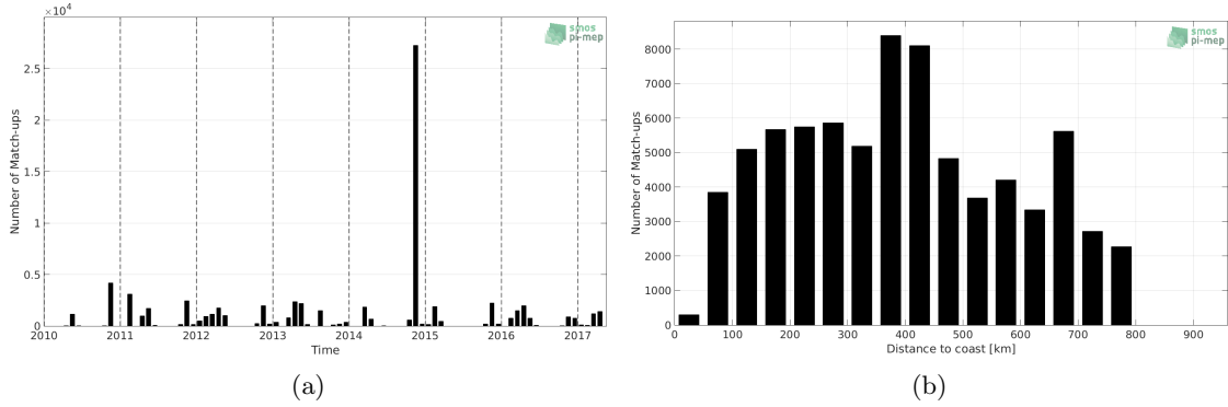
Figure 1: Number of match-ups between TSG-POLARSTERN and SMOS-L3-CATDS-IFREMER-CECOS-V2-MONTHLY-0.25DEG SSS as a function of time (a) and as function of the distance to coast (b) over the SMOS coastal zone ( \geq 800\text{km} ) 60N-60S Pi-MEP region and for the full satellite product period.
