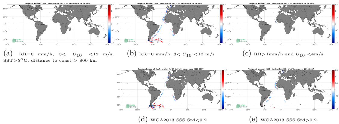
Figure 12: Temporal mean gridded over spatial boxes of size 1^\circ \times 1^\circ of \Delta SSS (SMOS-L3-CATDS-IFREMER-CECOS-V2-MONTHLY-0.25DEG - TSG-POLARSTERN) for 5 different subdatasets corresponding to:RR=0 mm/h, 3 < U_{10} < 12 m/s, SST >5^\circ C, distance to coast > 800 km (a), RR=0 mm/h, 3 < U_{10} < 12 m/s (b), RR >1 mm/h and U_{10} < 4 m/s (c), WOA2013 SSS Std <0.2 (d), WOA2013 SSS Std >0.2 (e).
