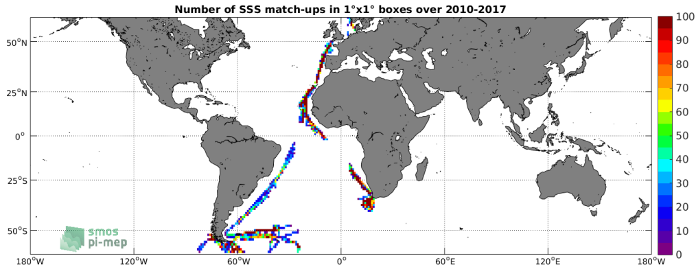
Figure 4: Number of SSS match-ups between TSG-POLARSTERN SSS and the SMOS-L3-CATDS-IFREMER-CECOS-V2-MONTHLY-0.25DEG SSS product for the SMOS coastal zone ( \pm 800\text{km} ) 60N-60S Pi-MEP region over 1^\circ \times 1^\circ boxes and for the full satellite product period.
