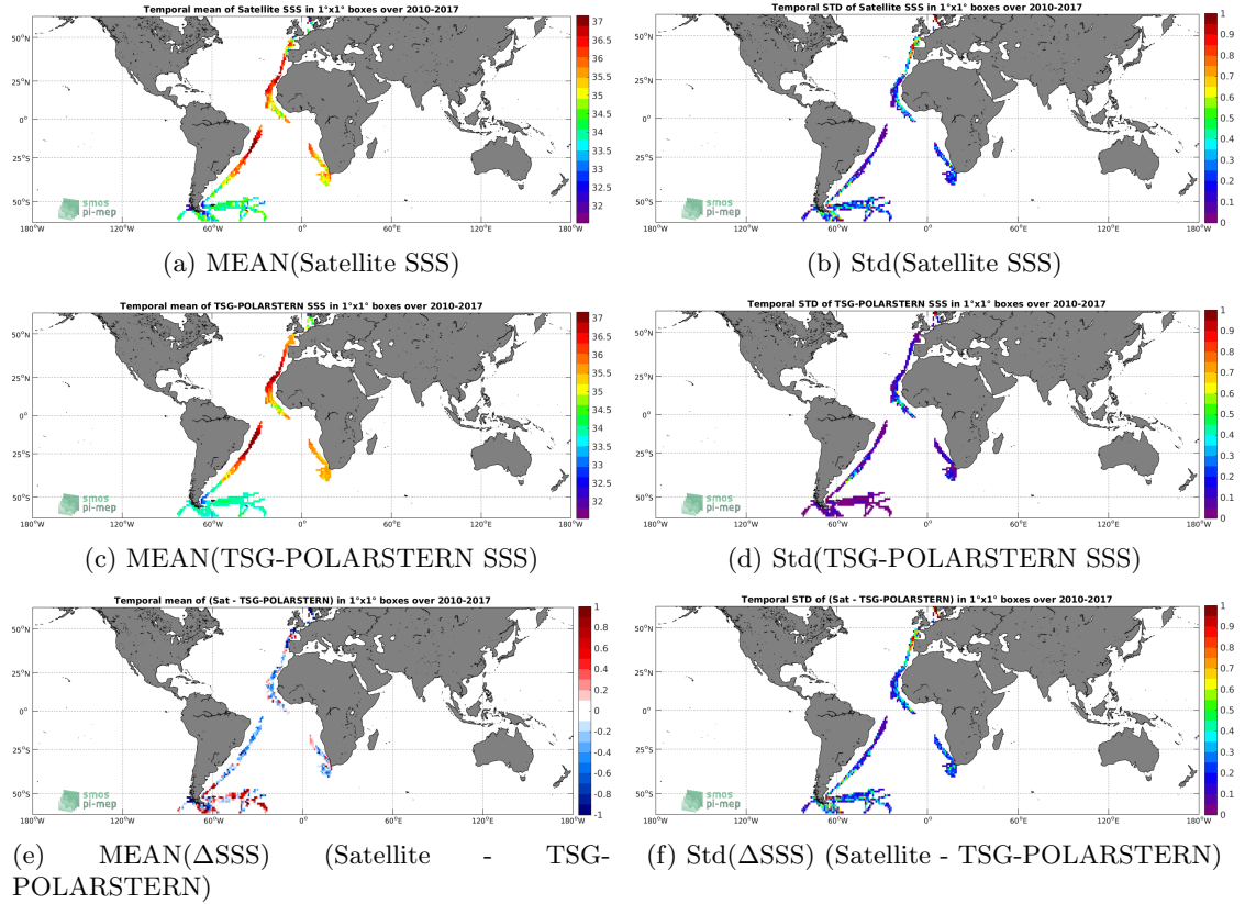
Figure 6: Temporal mean (left) and Std (right) of SSS from SMOS-L3-CATDS-IFREMER-CECOS-V2-MONTHLY-0.25DEG (top), TSG-POLARSTERN (middle), and of \Delta SSS (Satellite - TSG-POLARSTERN). Only match-up pairs are used to generate these maps.
