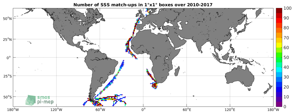
Figure 4: Number of SSS match-ups between TSG-POLARSTERN SSS and the SMOS-L3-CATDS-IFREMER-CECOS-V2-MONTHLY-0.25DEG SSS product for the SMOS coastal zone ( \approx 800\text{km} ) 60N-60S Pi-MEP region over 1^\circ \times 1^\circ boxes and for the full satellite product period.
