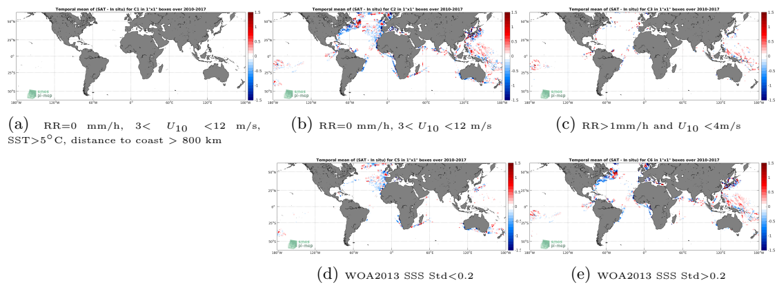
Figure 12: Temporal mean gridded over spatial boxes of size 1^\circ \times 1^\circ of \Delta SSS (SMOS SSS L3 v2 - Monthly - 0.25 Deg (CATDS-CECOS-IFREMER) - TSG (LEGOS-DM)) for 5 different subdatasets corresponding to:RR=0 mm/h, 3 < U_{10} < 12 m/s, SST >5^\circ C, distance to coast > 800 km (a), RR=0 mm/h, 3 < U_{10} < 12 m/s (b), RR >1 mm/h and U_{10} < 4 m/s (c), WOA2013 SSS Std <0.2 (d), WOA2013 SSS Std >0.2 (e).
