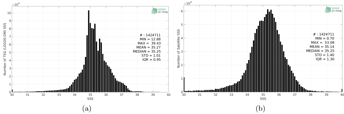
Figure 2: Histograms of SSS from TSG (LEGOS-DM) (a) and SMOS SSS L3 v2 - Monthly - 0.25 Deg (CATDS-CECOS-IFREMER) (b) considering all match-up pairs per bins of 0.1 over the SMOS coastal zone (<800km) 60N-60S Pi-MEP region and for the full satellite product period.
