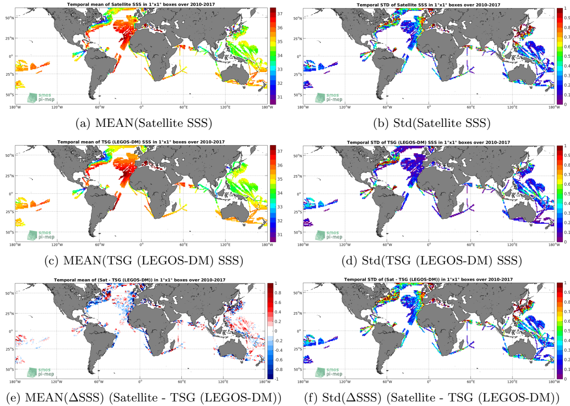
Figure 6: Temporal mean (left) and Std (right) of SSS from SMOS SSS L3 v2 - Monthly - 0.25 Deg (CATDS-CECOS-IFREMER) (top), TSG (LEGOS-DM) (middle), and of \Delta SSS (Satellite - TSG (LEGOS-DM)). Only match-up pairs are used to generate these maps.
