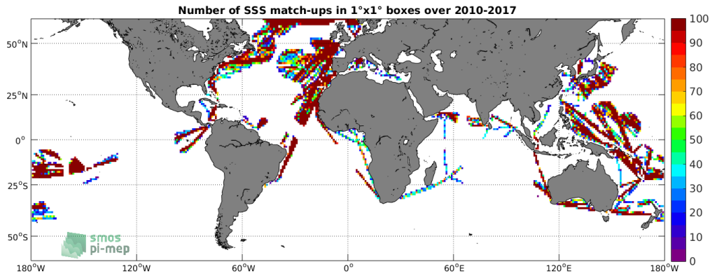
Figure 4: Number of SSS match-ups between TSG (LEGOS-DM) SSS and the SMOS SSS L3 v2 - Monthly - 0.25 Deg (CATDS-CECOS-IFREMER) SSS product for the SMOS coastal zone (<800km) 60N-60S Pi-MEP region over 1^\circ \times 1^\circ boxes and for the full satellite product period.
