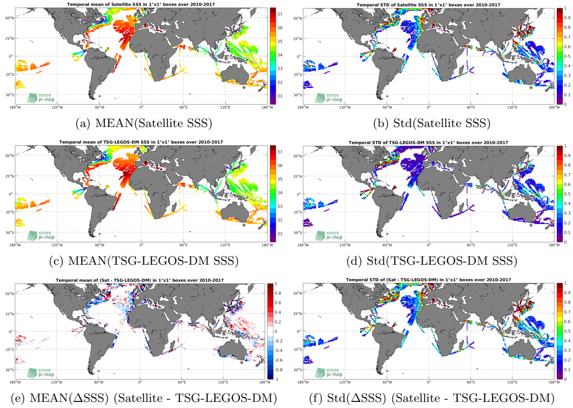
Figure 6: Temporal mean (left) and Std (right) of SSS from SMOS L3 v2 - Monthly - 0.25 Deg (CATDS-CECOS-IFREMER) (top), TSG-LEGOS-DM (middle), and of \Delta SSS (Satellite - TSG-LEGOS-DM). Only match-up pairs are used to generate these maps.
