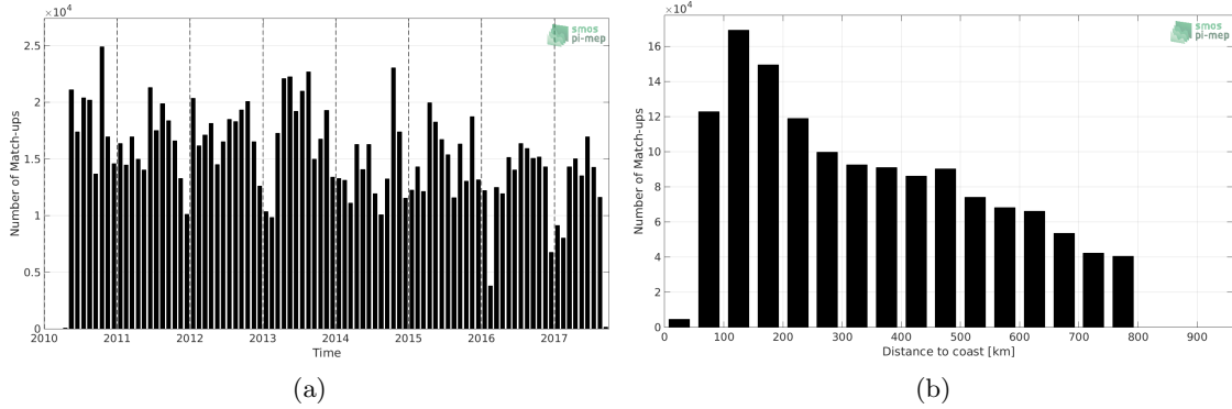
Figure 1: Number of match-ups between TSG-LEGOS-DM and SMOS L3 v2 - Monthly - 0.25 Deg (CATDS-CECOS-IFREMER) SSS as a function of time (a) and as function of the distance to coast (b) over the SMOS coastal zone (<800km) 60N-60S Pi-MEP region and for the full satellite product period.
