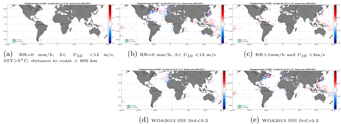
Figure 12: Temporal mean gridded over spatial boxes of size 1^\circ \times 1^\circ of \Delta SSS (SMOS L3 v2 - Monthly - 0.25 Deg (CATDS-CECOS-IFREMER) - TSG-LEGOS-DM) for 5 different subdatasets corresponding to:RR=0 mm/h, 3 < U_{10} < 12 m/s, SST >5^\circ\text{C} , distance to coast > 800 km (a), RR=0 mm/h, 3 < U_{10} < 12 m/s (b), RR >1 mm/h and U_{10} < 4 m/s (c), WOA2013 SSS Std <0.2 (d), WOA2013 SSS Std >0.2 (e).
