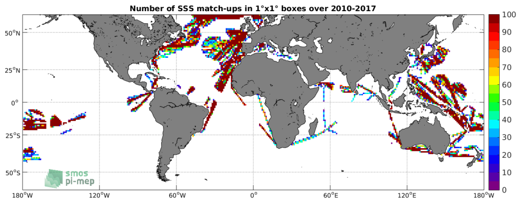
Figure 4: Number of SSS match-ups between TSG-LEGOS-DM SSS and the SMOS L3 v2 - Monthly - 0.25 Deg (CATDS-CECOS-IFREMER) SSS product for the SMOS coastal zone (<800km) 60N-60S Pi-MEP region over 1^\circ \times 1^\circ boxes and for the full satellite product period.
