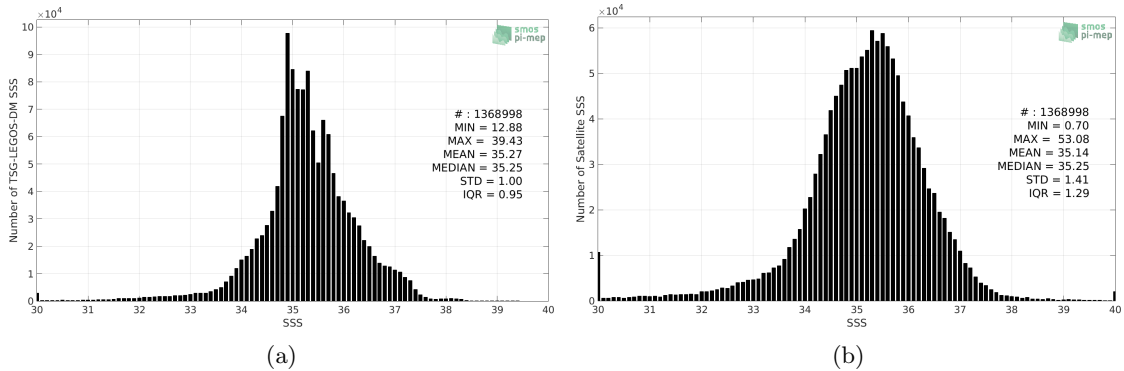
Figure 2: Histograms of SSS from TSG-LEGOS-DM (a) and SMOS L3 v2 - Monthly - 0.25 Deg (CATDS-CECOS-IFREMER) (b) considering all match-up pairs per bins of 0.1 over the SMOS coastal zone (<800km) 60N-60S Pi-MEP region and for the full satellite product period.
