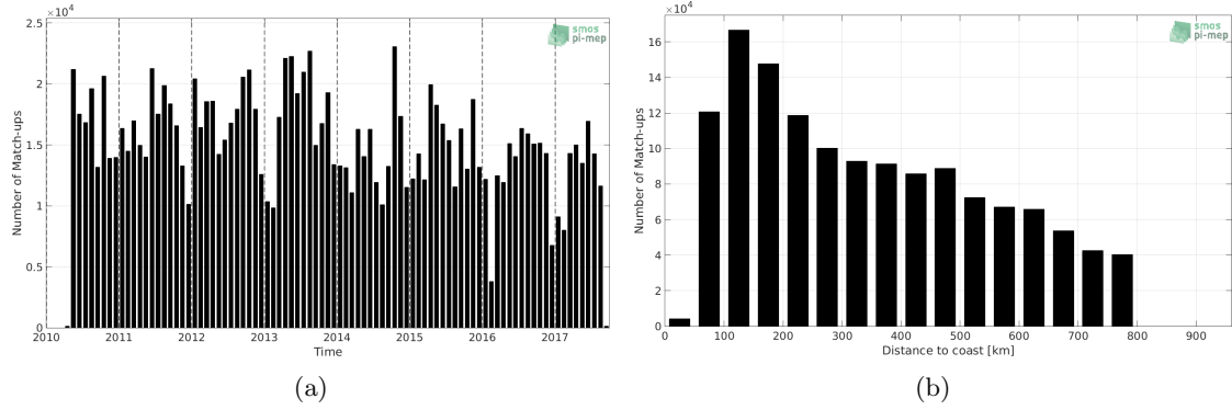
Figure 1: Number of match-ups between TSG-LEGOS-DM and SMOS-L3-CATDS-IFREMER-CECOS-V2-MONTHLY-0.25DEG SSS as a function of time (a) and as function of the distance to coast (b) over the SMOS coastal zone ( \approx 800\text{km} ) 60N-60S Pi-MEP region and for the full satellite product period.
