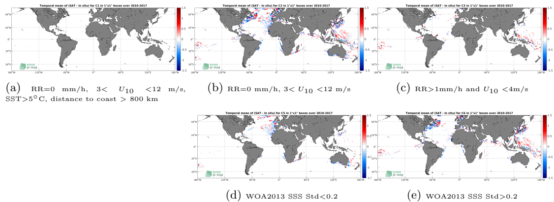
Figure 12: Temporal mean gridded over spatial boxes of size 1^\circ \times 1^\circ of \Delta SSS (SMOS-L3-CATDS-IFREMER-CECOS-V2-MONTHLY-0.25DEG - TSG-LEGOS-DM) for 5 different subdatasets corresponding to:RR=0 mm/h, 3 < U_{10} < 12 m/s, SST >5^\circ C, distance to coast > 800 km (a), RR=0 mm/h, 3 < U_{10} < 12 m/s (b), RR >1 mm/h and U_{10} < 4 m/s (c), WOA2013 SSS Std <0.2 (d), WOA2013 SSS Std >0.2 (e).
