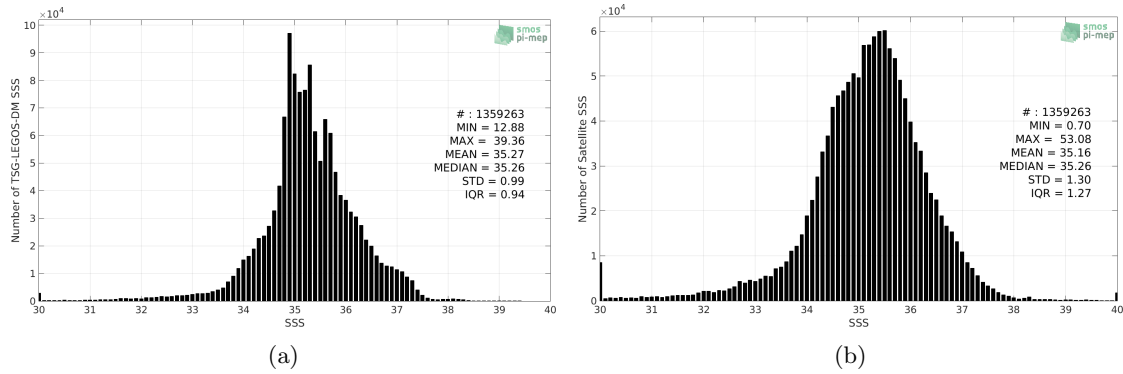
Figure 2: Histograms of SSS from TSG-LEGOS-DM (a) and SMOS-L3-CATDS-IFREMER-CECOS-V2-MONTHLY-0.25DEG (b) considering all match-up pairs per bins of 0.1 over the SMOS coastal zone ( \approx 800\text{km} ) 60N-60S Pi-MEP region and for the full satellite product period.
