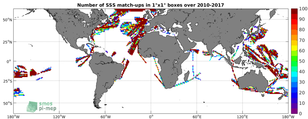
Figure 4: Number of SSS match-ups between TSG-LEGOS-DM SSS and the SMOS-L3-CATDS-IFREMER-CECOS-V2-MONTHLY-0.25DEG SSS product for the SMOS coastal zone ( \approx 800\text{km} ) 60N-60S Pi-MEP region over 1^\circ \times 1^\circ boxes and for the full satellite product period.
