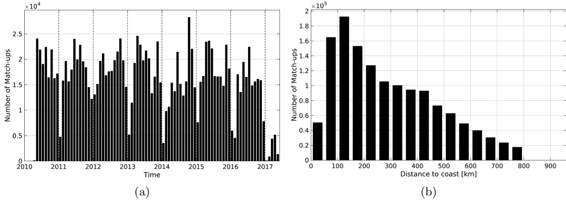
Figure 1: Number of match-ups between TSG-LEGOS-DM and SMOS-L3-CATDS-IFREMER-CECOS-V2-MONTHLY-0.25DEG SSS as a function of time (a) and as function of the distance to coast (b) over the SMOS coastal zone ( \geq 800 km) 60N-60S Pi-MEP region and for the full satellite product period.
