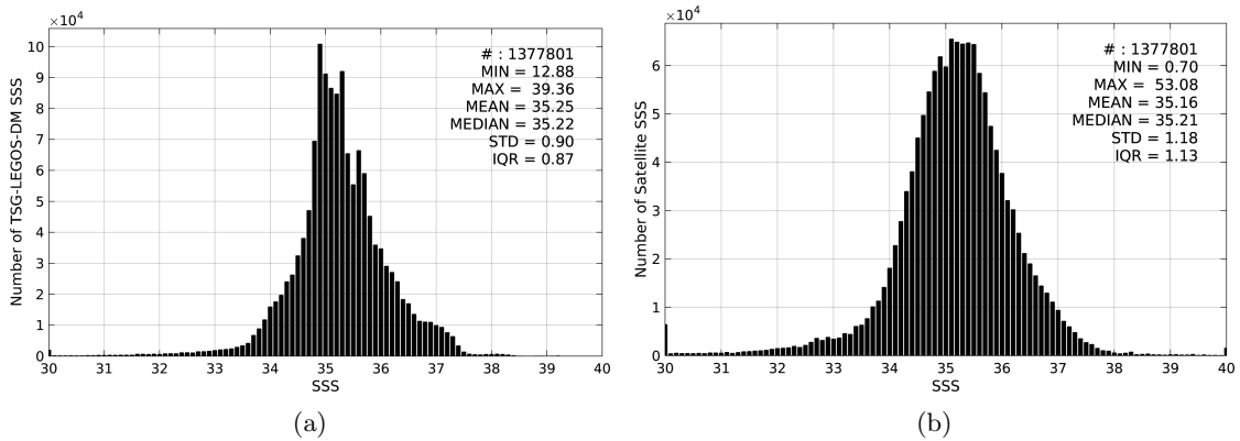
Figure 2: Histograms of SSS from TSG-LEGOS-DM (a) and SMOS-L3-CATDS-IFREMER-CECOS-V2-MONTHLY-0.25DEG (b) considering all match-up pairs per bins of 0.1 over the SMOS coastal zone ( \geq 800 km) 60N-60S Pi-MEP region and for the full satellite product period.
