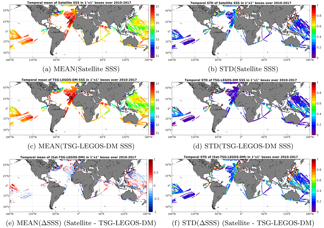
Figure 6: Temporal mean (left) and STD (right) of SSS from SMOS-L3-CATDS-IFREMER-CECOS-V2-MONTHLY-0.25DEG (top), TSG-LEGOS-DM (middle), and of \Delta SSS (Satellite - TSG-LEGOS-DM). Only match-up pairs are used to generate these maps.
