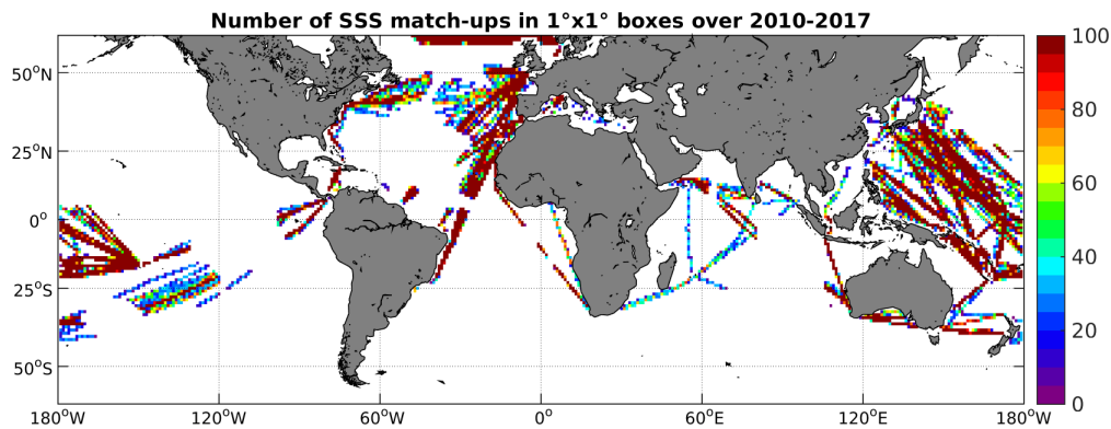
Figure 4: Number of SSS match-ups between TSG-LEGOS-DM SSS and the SMOS-L3-CATDS-IFREMER-CECOS-V2-MONTHLY-0.25DEG SSS product for the SMOS coastal zone ( \pm 800\text{km} ) 60N-60S Pi-MEP region over 1^\circ \times 1^\circ boxes and for the full satellite product period.
