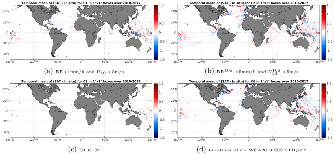
Figure 12: Temporal mean gridded over spatial boxes of size 1^\circ \times 1^\circ of \Delta SSS (SMOS-L3-CATDS-IFREMER-CECOS-V2-MONTHLY-0.25DEG - TSG-LEGOS-DM) for 4 different subdatasets corresponding to: RR > 1\text{mm/h} and U_{10} < 5\text{m/s} (a), RR^{10d} > 5\text{mm/h} and U_{10}^{10d} < 5\text{m/s} (b), C1 U C2 (c), Locations where WOA2013 SSS STD > 0.2 (d).
