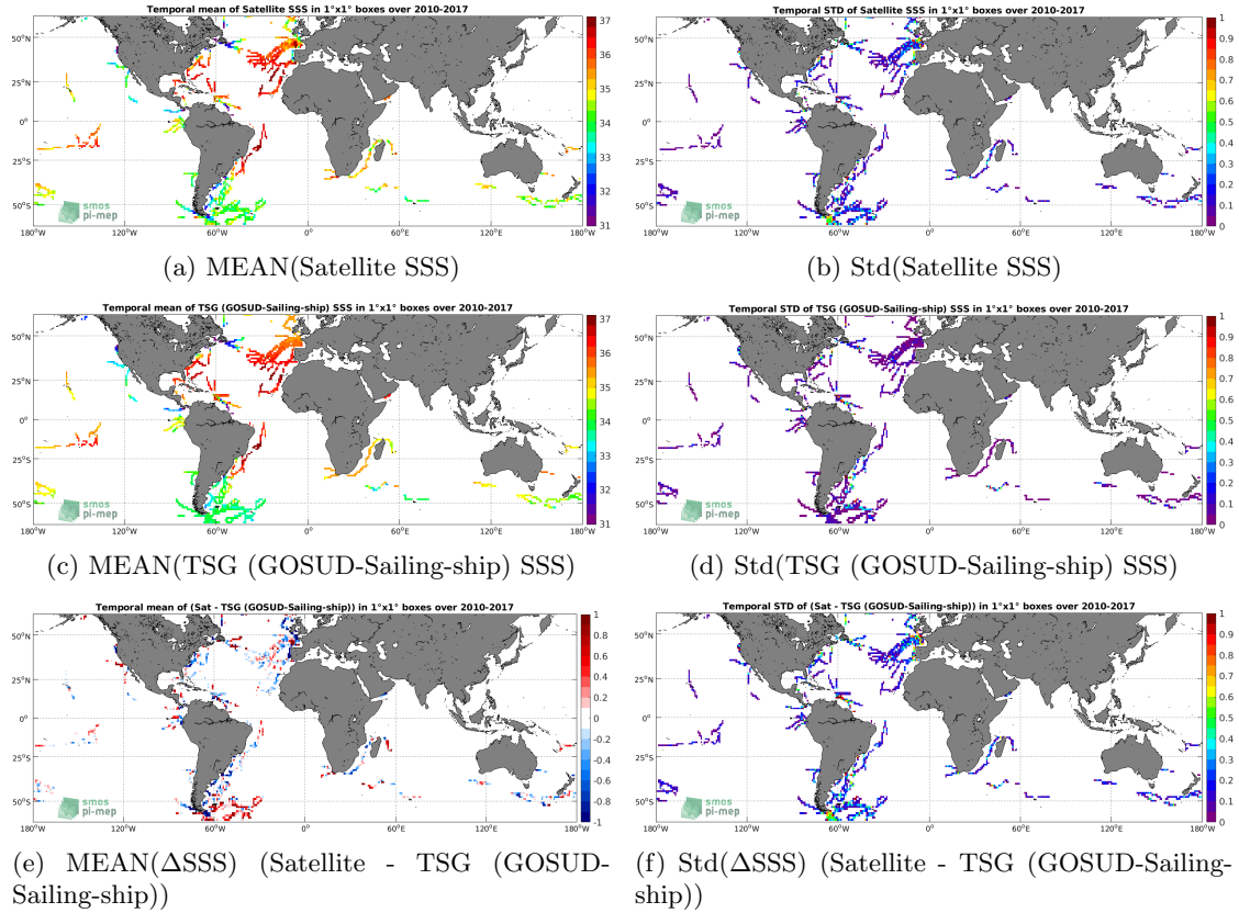
Figure 6: Temporal mean (left) and Std (right) of SSS from SMOS SSS L3 v2 - Monthly - 0.25 Deg (CATDS-CECOS-IFREMER) (top), TSG (GOSUD-Sailing-ship) (middle), and of \Delta SSS (Satellite - TSG (GOSUD-Sailing-ship)). Only match-up pairs are used to generate these maps.
