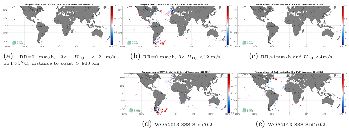
Figure 12: Temporal mean gridded over spatial boxes of size 1^\circ \times 1^\circ of \Delta SSS (SMOS SSS L3 v2 - Monthly - 0.25 Deg (CATDS-CECOS-IFREMER) - TSG (GOSUD-Sailing-ship)) for 5 different subdatasets corresponding to:RR=0 mm/h, 3 < U_{10} < 12 m/s, SST >5^\circ\text{C} , distance to coast > 800 km (a), RR=0 mm/h, 3 < U_{10} < 12 m/s (b), RR >1 mm/h and U_{10} < 4 m/s (c), WOA2013 SSS Std <0.2 (d), WOA2013 SSS Std >0.2 (e).
