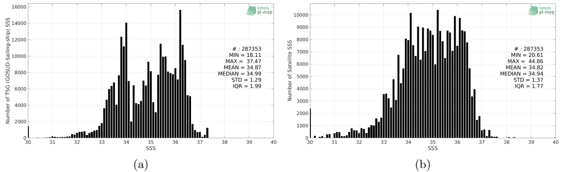
Figure 2: Histograms of SSS from TSG (GOSUD-Sailing-ship) (a) and SMOS SSS L3 v2 - Monthly - 0.25 Deg (CATDS-CECOS-IFREMER) (b) considering all match-up pairs per bins of 0.1 over the SMOS coastal zone (<800km) 60N-60S Pi-MEP region and for the full satellite product period.
