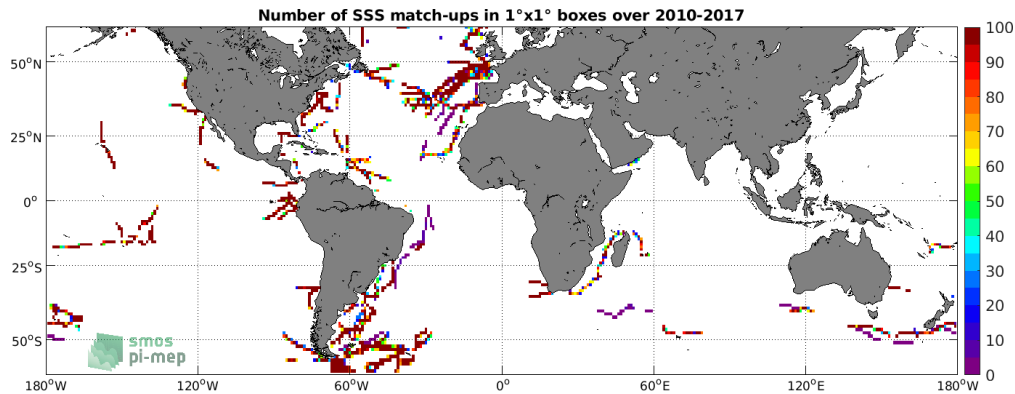
Figure 4: Number of SSS match-ups between TSG (GOSUD-Sailing-ship) SSS and the SMOS SSS L3 v2 - Monthly - 0.25 Deg (CATDS-CECOS-IFREMER) SSS product for the SMOS coastal zone (<800km) 60N-60S Pi-MEP region over 1^\circ \times 1^\circ boxes and for the full satellite product period.
