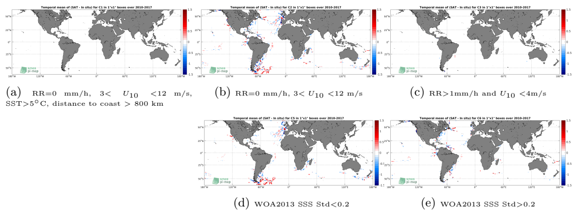
Figure 12: Temporal mean gridded over spatial boxes of size 1^\circ \times 1^\circ of \Delta\text{SSS} (SMOS SSS L3 v2 - Monthly - 0.25 Deg (CATDS-CECOS-IFREMER) - TSG (GOSUD-Sailing-ship)) for 5 different subdatasets corresponding to: RR=0 mm/h, 3 < U_{10} < 12 m/s, SST > 5°C, distance to coast > 800 km (a), RR=0 mm/h, 3 < U_{10} < 12 m/s (b), RR > 1mm/h and U_{10} < 4 m/s (c), WOA2013 SSS Std < 0.2 (d), WOA2013 SSS Std > 0.2 (e).
