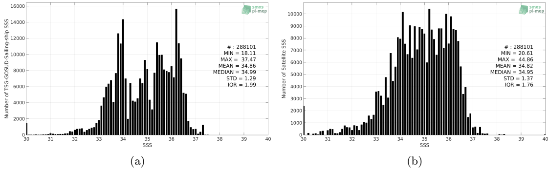
Figure 2: Histograms of SSS from TSG-GOSUD-Sailing-ship (a) and SMOS-L3-CATDS-IFREMER-CECOS-V2-MONTHLY-0.25DEG (b) considering all match-up pairs per bins of 0.1 over the SMOS coastal zone ( \leq 800 km) 60N-60S Pi-MEP region and for the full satellite product period.
