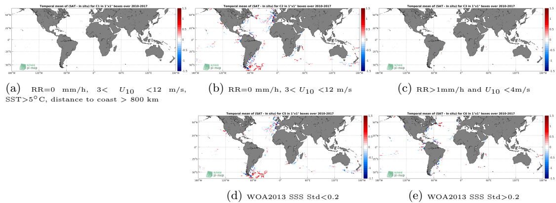
Figure 12: Temporal mean gridded over spatial boxes of size 1^\circ \times 1^\circ of \Delta SSS (SMOS-L3-CATDS-IFREMER-CECOS-V2-MONTHLY-0.25DEG - TSG-GOSUD-Sailing-ship) for 5 different sub-datasets corresponding to: RR=0 mm/h, 3 < U_{10} < 12 m/s, SST >5^\circ\text{C} , distance to coast > 800 km (a), RR=0 mm/h, 3 < U_{10} < 12 m/s (b), RR >1 mm/h and U_{10} < 4 m/s (c), WOA2013 SSS Std <0.2 (d), WOA2013 SSS Std >0.2 (e).
