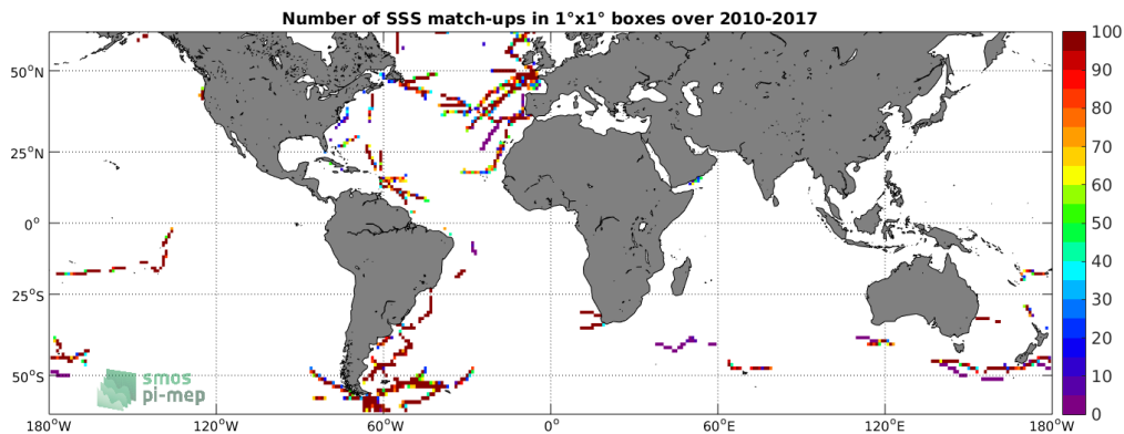
Figure 4: Number of SSS match-ups between TSG-GOSUD-Sailing-ship SSS and the SMOS-L3-CATDS-IFREMER-CECOS-V2-MONTHLY-0.25DEG SSS product for the SMOS coastal zone ( \approx 800 km) 60N-60S Pi-MEP region over 1^\circ \times 1^\circ boxes and for the full satellite product period.
