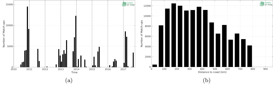
Figure 1: Number of match-ups between TSG-GOSUD-Sailing-ship and SMOS-L3-CATDS-IFREMER-CECOS-V2-MONTHLY-0.25DEG SSS as a function of time (a) and as function of the distance to coast (b) over the SMOS coastal zone ( \approx 800\text{km} ) 60N-60S Pi-MEP region and for the full satellite product period.
