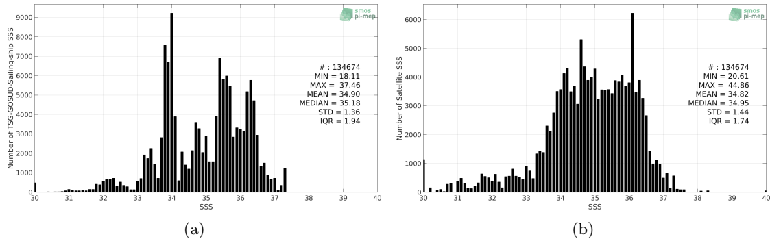
Figure 2: Histograms of SSS from TSG-GOSUD-Sailing-ship (a) and SMOS-L3-CATDS-IFREMER-CECOS-V2-MONTHLY-0.25DEG (b) considering all match-up pairs per bins of 0.1 over the SMOS coastal zone ( \approx 800\text{km} ) 60N-60S Pi-MEP region and for the full satellite product period.
