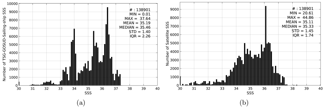
Figure 2: Histograms of SSS from TSG-GOSUD-Sailing-ship (a) and SMOS-L3-CATDS-IFREMER-CECOS-V2-MONTHLY-0.25DEG (b) considering all match-up pairs per bins of 0.1 over the SMOS coastal zone ( \geq 800\text{km} ) 60N-60S Pi-MEP region and for the full satellite product period.
