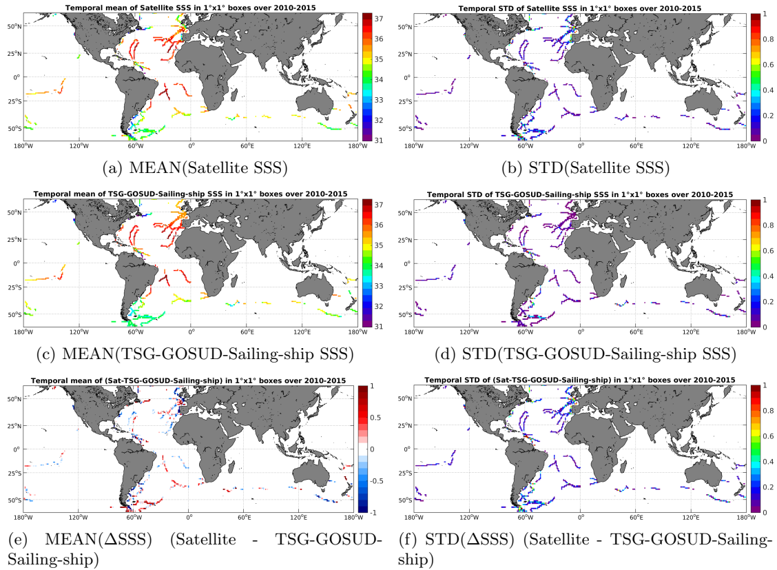
Figure 6: Temporal mean (left) and STD (right) of SSS from SMOS-L3-CATDS-IFREMER-CECOS-V2-MONTHLY-0.25DEG (top), TSG-GOSUD-Sailing-ship (middle), and of \Delta SSS (Satellite - TSG-GOSUD-Sailing-ship). Only match-up pairs are used to generate these maps.
