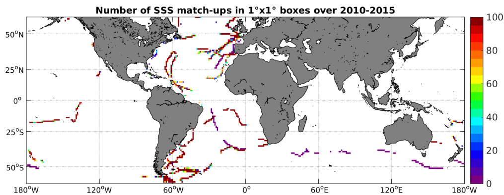
Figure 4: Number of SSS match-ups between TSG-GOSUD-Sailing-ship SSS and the SMOS-L3-CATDS-IFREMER-CECOS-V2-MONTHLY-0.25DEG SSS product for the SMOS coastal zone ( \pm 800\text{km} ) 60N-60S Pi-MEP region over 1^\circ \times 1^\circ boxes and for the full satellite product period.
