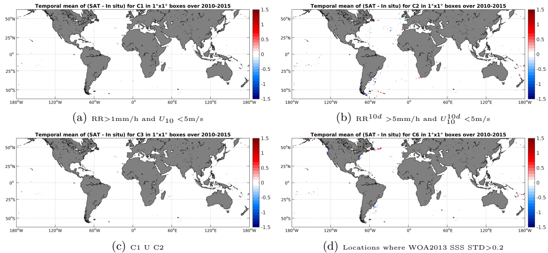
Figure 12: Temporal mean gridded over spatial boxes of size 1^\circ \times 1^\circ of \Delta SSS (SMOS-L3-CATDS-IFREMER-CECOS-V2-MONTHLY-0.25DEG - TSG-GOSUD-Sailing-ship) for 4 different sub-datasets corresponding to: RR > 1\text{mm/h} and U_{10} < 5\text{m/s} (a), RR^{10d} > 5\text{mm/h} and U_{10}^{10d} < 5\text{m/s} (b), C1 U C2 (c), Locations where WOA2013 SSS STD > 0.2 (d).
