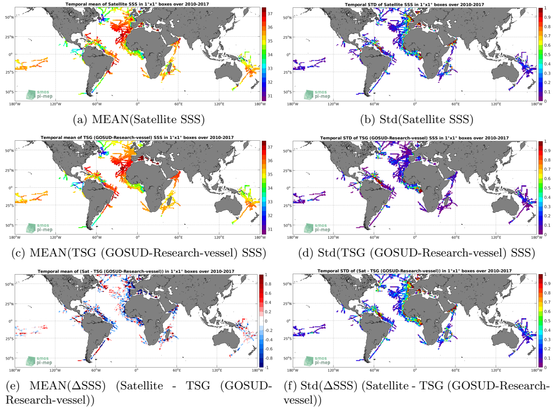
Figure 6: Temporal mean (left) and Std (right) of SSS from SMOS SSS L3 v2 - Monthly - 0.25 Deg (CATDS-CECOS-IFREMER) (top), TSG (GOSUD-Research-vessel) (middle), and of \Delta SSS (Satellite - TSG (GOSUD-Research-vessel)). Only match-up pairs are used to generate these maps.
