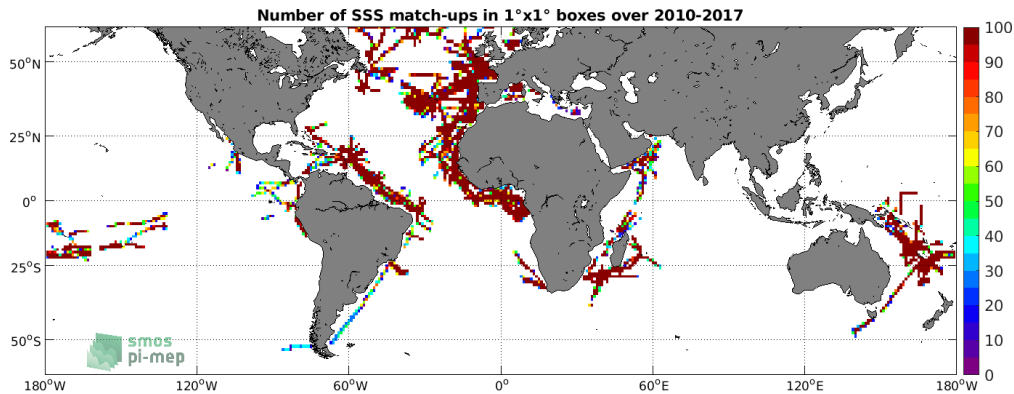
Figure 4: Number of SSS match-ups between TSG (GOSUD-Research-vessel) SSS and the SMOS SSS L3 v2 - Monthly - 0.25 Deg (CATDS-CECOS-IFREMER) SSS product for the SMOS coastal zone (<800km) 60N-60S Pi-MEP region over 1°x1° boxes and for the full satellite product period.
