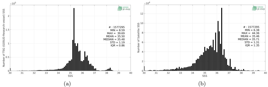
Figure 2: Histograms of SSS from TSG (GOSUD-Research-vessel) (a) and SMOS SSS L3 v2 - Monthly - 0.25 Deg (CATDS-CECOS-IFREMER) (b) considering all match-up pairs per bins of 0.1 over the SMOS coastal zone (<800km) 60N-60S Pi-MEP region and for the full satellite product period.
