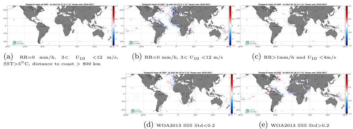
Figure 12: Temporal mean gridded over spatial boxes of size 1^\circ \times 1^\circ of \Delta SSS (SMOS SSS L3 v2 - Monthly - 0.25 Deg (CATDS-CECOS-IFREMER) - TSG (GOSUD-Research-vessel)) for 5 different subdatasets corresponding to:RR=0 mm/h, 3 < U_{10} < 12 m/s, SST >5^\circ\text{C} , distance to coast > 800 km (a), RR=0 mm/h, 3 < U_{10} < 12 m/s (b), RR >1 mm/h and U_{10} < 4 m/s (c), WOA2013 SSS Std <0.2 (d), WOA2013 SSS Std >0.2 (e).
