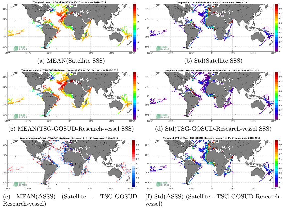
Figure 6: Temporal mean (left) and Std (right) of SSS from SMOS L3 v2 - Monthly - 0.25 Deg (CATDS-CECOS-IFREMER) (top), TSG-GOSUD-Research-vessel (middle), and of \Delta SSS (Satellite - TSG-GOSUD-Research-vessel). Only match-up pairs are used to generate these maps.
