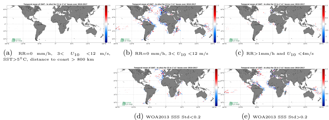
Figure 12: Temporal mean gridded over spatial boxes of size 1^\circ \times 1^\circ of \Delta SSS (SMOS L3 v2 - Monthly - 0.25 Deg (CATDS-CECOS-IFREMER) - TSG-GOSUD-Research-vessel) for 5 different subdatasets corresponding to:RR=0 mm/h, 3 < U_{10} < 12 m/s, SST > 5^\circ\text{C} , distance to coast > 800 km (a), RR=0 mm/h, 3 < U_{10} < 12 m/s (b), RR > 1 mm/h and U_{10} < 4 m/s (c), WOA2013 SSS Std < 0.2 (d), WOA2013 SSS Std > 0.2 (e).
