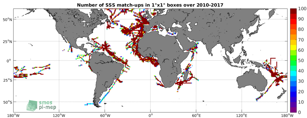
Figure 4: Number of SSS match-ups between TSG-GOSUD-Research-vessel SSS and the SMOS L3 v2 - Monthly - 0.25 Deg (CATDS-CECOS-IFREMER) SSS product for the SMOS coastal zone (<800km) 60N-60S Pi-MEP region over 1°x1° boxes and for the full satellite product period.
