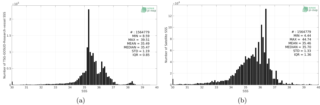
Figure 2: Histograms of SSS from TSG-GOSUD-Research-vessel (a) and SMOS L3 v2 - Monthly - 0.25 Deg (CATDS-CECOS-IFREMER) (b) considering all match-up pairs per bins of 0.1 over the SMOS coastal zone (<800km) 60N-60S Pi-MEP region and for the full satellite product period.
