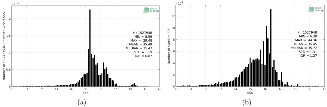
Figure 2: Histograms of SSS from TSG-GOSUD-Research-vessel (a) and SMOS-L3-CATDS-IFREMER-CECOS-V2-MONTHLY-0.25DEG (b) considering all match-up pairs per bins of 0.1 over the SMOS coastal zone ( \geq 800 km) 60N-60S Pi-MEP region and for the full satellite product period.
