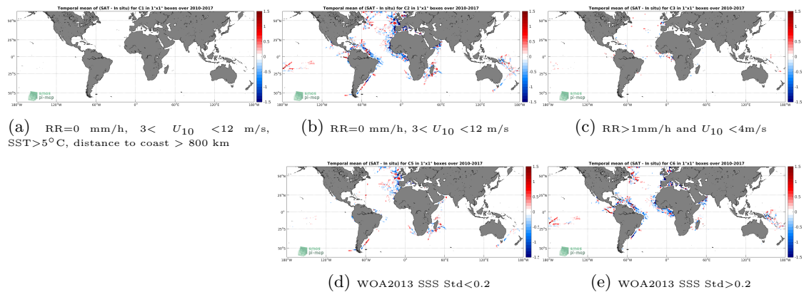
Figure 12: Temporal mean gridded over spatial boxes of size 1^\circ \times 1^\circ of \Delta SSS (SMOS-L3-CATDS-IFREMER-CECOS-V2-MONTHLY-0.25DEG - TSG-GOSUD-Research-vessel) for 5 different subdatasets corresponding to:RR=0 mm/h, 3 < U_{10} < 12 m/s, SST >5^\circ C, distance to coast > 800 km (a), RR=0 mm/h, 3 < U_{10} < 12 m/s (b), RR >1 mm/h and U_{10} < 4 m/s (c), WOA2013 SSS Std <0.2 (d), WOA2013 SSS Std >0.2 (e).
