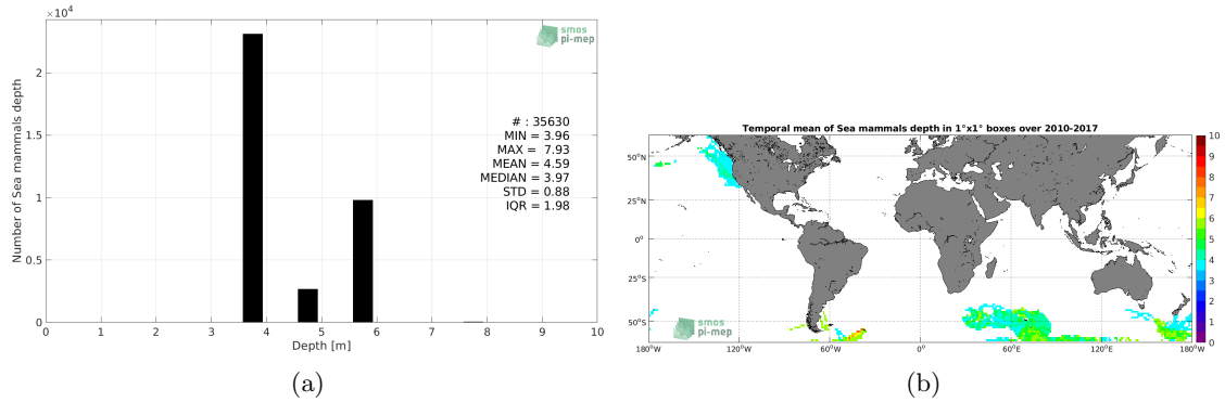
Figure 3: Histograms of the depth of the upper level SSS measurements from Sea mammals in the Match-up DataBase for the SMOS coastal zone ( <800\text{km} ) 60N-60S Pi-MEP region (a) and temporal mean spatial distribution of pressure of the in situ SSS data over 1^\circ \times 1^\circ boxes and for the full satellite product period (b).
