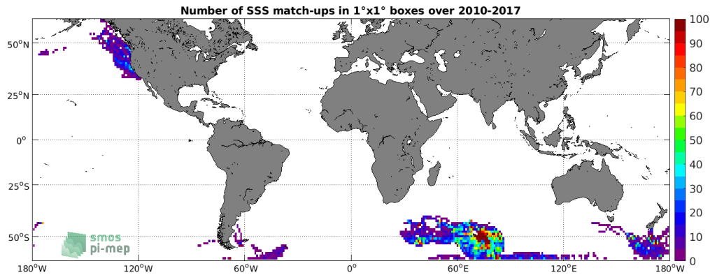
Figure 4: Number of SSS match-ups between Sea mammals SSS and the SMOS SSS L3 v2 - Monthly - 0.25 Deg (CATDS-CECOS-IFREMER) SSS product for the SMOS coastal zone ( <800\text{km} ) 60N-60S Pi-MEP region over 1^\circ \times 1^\circ boxes and for the full satellite product period.
