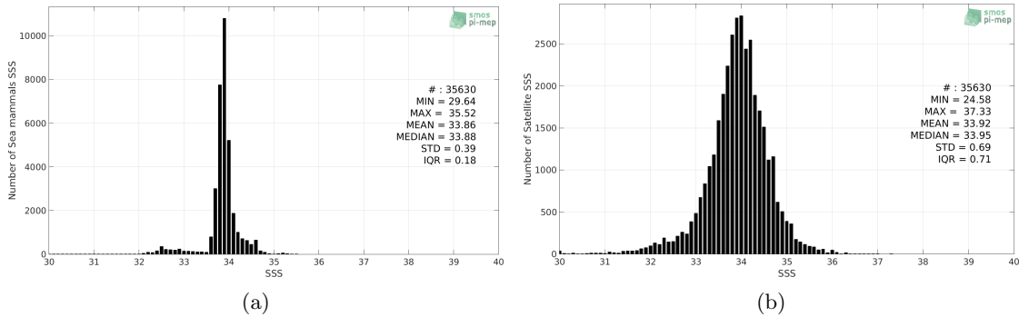
Figure 2: Histograms of SSS from Sea mammals (a) and SMOS-L3-CATDS-IFREMER-CECOS-V2-MONTHLY-0.25DEG (b) considering all match-up pairs per bins of 0.1 over the SMOS coastal zone ( \leq 800 km) 60N-60S Pi-MEP region and for the full satellite product period.
