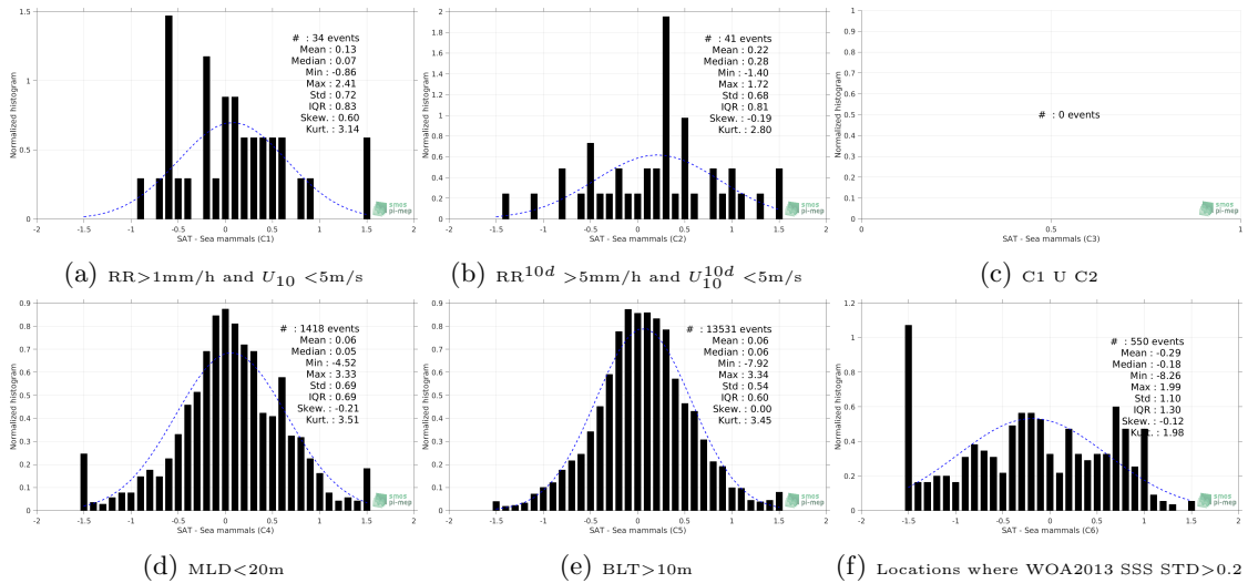
Figure 13: Normalized histogram of \Delta\text{SSS} (SMOS-L3-CATDS-IFREMER-CECOS-V2-MONTHLY-0.25DEG - Sea mammals) for 6 different subdatasets corresponding to: \text{RR} > 1\text{mm/h} and U_{10} < 5\text{m/s} (a), \text{RR}^{10d} > 5\text{mm/h} and U_{10}^{10d} < 5\text{m/s} (b), C1 U C2 (c), \text{MLD} < 20\text{m} (d), \text{BLT} > 10\text{m} (e), Locations where WOA2013 SSS \text{STD} > 0.2 (f).
