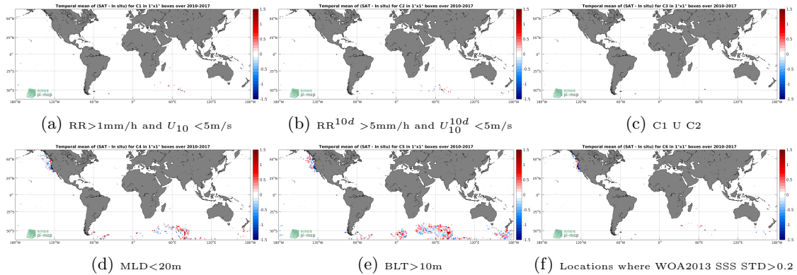
Figure 12: Temporal mean gridded over spatial boxes of size 1^\circ \times 1^\circ of \Delta\text{SSS} (SMOS-L3-CATDS-IFREMER-CECOS-V2-MONTHLY-0.25DEG - Sea mammals) for 6 different subdatasets corresponding to: \text{RR} > 1\text{mm/h} and U_{10} < 5\text{m/s} (a), \text{RR}^{10d} > 5\text{mm/h} and U_{10}^{10d} < 5\text{m/s} (b), C1 U C2 (c), \text{MLD} < 20\text{m} (d), \text{BLT} > 10\text{m} (e), Locations where WOA2013 SSS \text{STD} > 0.2 (f).
