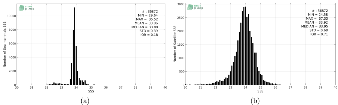
Figure 2: Histograms of SSS from Sea mammals (a) and SMOS-L3-CATDS-IFREMER-CECOS-V2-MONTHLY-0.25DEG (b) considering all match-up pairs per bins of 0.1 over the SMOS coastal zone ( \pm 800 km) 60N-60S Pi-MEP region and for the full satellite product period.
