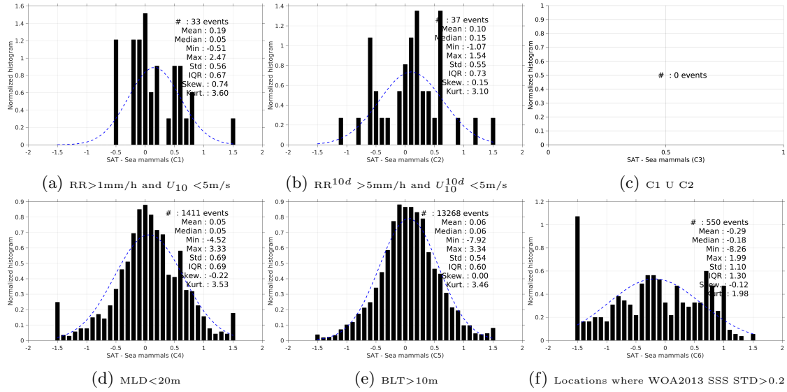
Figure 13: Normalized histogram of \Delta SSS (SMOS-L3-CATDS-IFREMER-CECOS-V2-MONTHLY-0.25DEG - Sea mammals) for 6 different subdatasets corresponding to: RR>1mm/h and U_{10} < 5\text{m/s} (a), RR^{10d} > 5\text{mm/h} and U_{10}^{10d} < 5\text{m/s} (b), C1 U C2 (c),MLD<20m (d),BLT>10m (e),Locations where WOA2013 SSS STD>0.2 (f).
