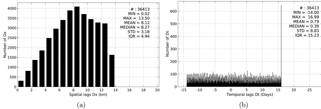
Figure 5: Histograms of the spatial (a) and temporal (b) lags between the time of the Sea mammals measurements and the date of the corresponding SMOS-L3-CATDS-IFREMER-CECOS-V2-MONTHLY-0.25DEG SSS product.
