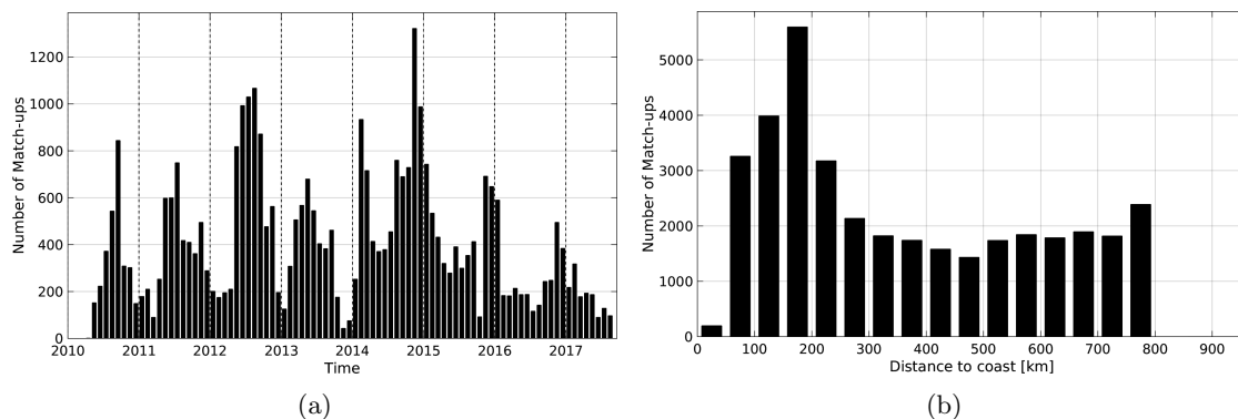
Figure 1: Number of match-ups between Sea mammals and SMOS-L3-CATDS-IFREMER-CECOS-V2-MONTHLY-0.25DEG SSS as a function of time (a) and as function of the distance to coast (b) over the SMOS coastal zone ( \pm 800 km) 60N-60S Pi-MEP region and for the full satellite product period.
