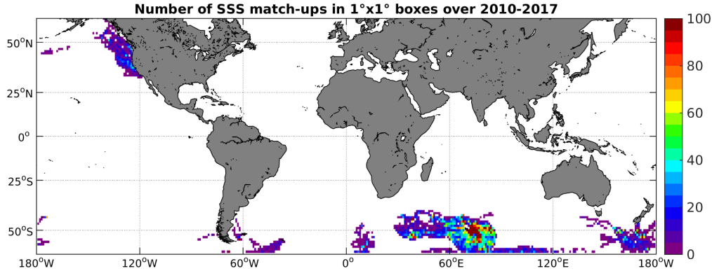
Figure 4: Number of SSS match-ups between Sea mammals SSS and the SMOS-L3-CATDS-IFREMER-CECOS-V2-MONTHLY-0.25DEG SSS product for the SMOS coastal zone ( \geq 800\text{km} ) 60N-60S Pi-MEP region over 1^\circ \times 1^\circ boxes and for the full satellite product period.
