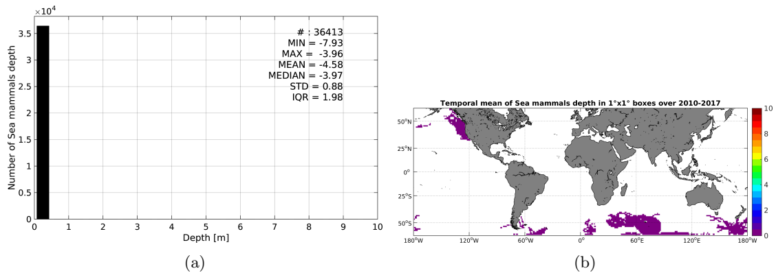
Figure 3: Histograms of the depth of the upper level SSS measurements from Sea mammals in the Match-up DataBase for the SMOS coastal zone ( \approx 800\text{km} ) 60N-60S Pi-MEP region (a) and temporal mean spatial distribution of pressure of the in situ SSS data over 1^\circ \times 1^\circ boxes and for the full satellite product period (b).
