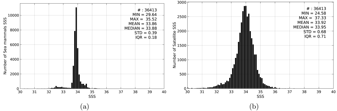
Figure 2: Histograms of SSS from Sea mammals (a) and SMOS-L3-CATDS-IFREMER-CECOS-V2-MONTHLY-0.25DEG (b) considering all match-up pairs per bins of 0.1 over the SMOS coastal zone ( \approx 800\text{km} ) 60N-60S Pi-MEP region and for the full satellite product period.
