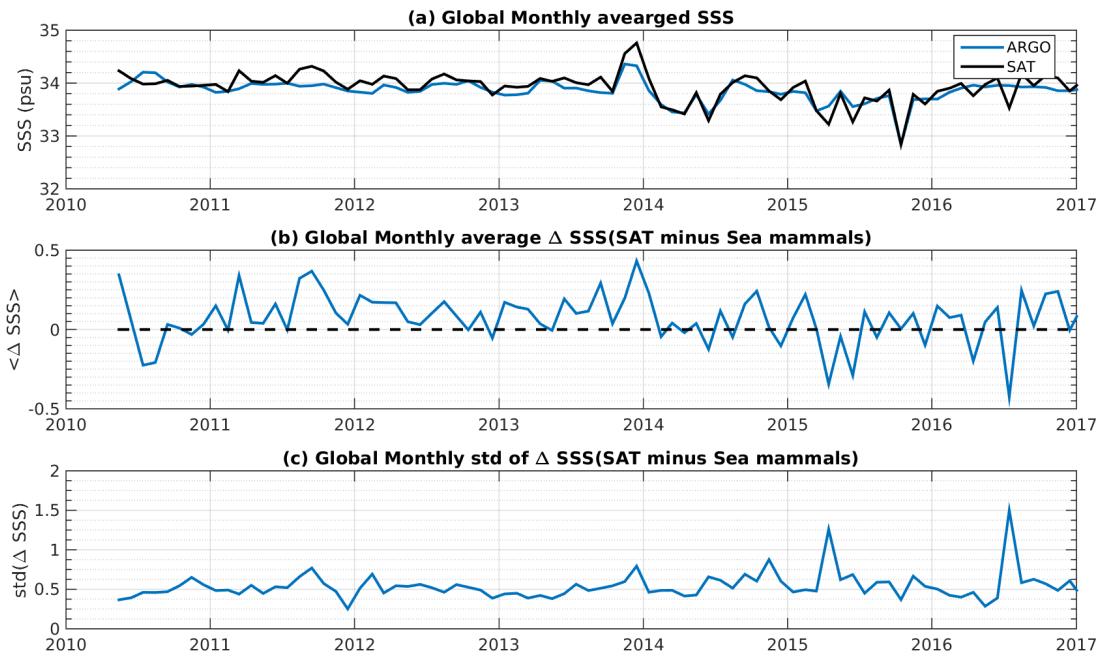
Figure 7: Time series of the monthly averaged mean SSS (top), mean \Delta SSS (Satellite - Sea mammals) and STD of \Delta SSS (Satellite - Sea mammals) over the SMOS coastal zone ( \pm 800 km) 60N-60S Pi-MEP region considering all match-ups collected by the Pi-MEP platform.
