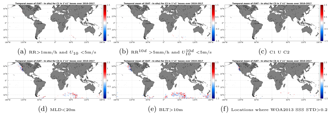
Figure 12: Temporal mean gridded over spatial boxes of size 1^\circ \times 1^\circ of \Delta SSS (SMOS-L3-CATDS-IFREMER-CECOS-V2-MONTHLY-0.25DEG - Sea mammals) for 6 different subdatasets corresponding to: RR > 1\text{mm/h} and U_{10} < 5\text{m/s} (a), RR^{10d} > 5\text{mm/h} and U_{10}^{10d} < 5\text{m/s} (b), C1 U C2 (c), MLD < 20m (d), BLT > 10m (e), Locations where WOA2013 SSS STD > 0.2 (f).
