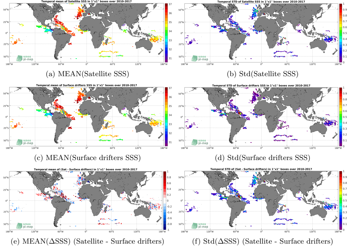
Figure 5: Temporal mean (left) and Std (right) of SSS from SMOS SSS L3 v2 - Monthly - 0.25 Deg (CATDS-CECOS-IFREMER) (top), Surface drifters (middle), and of \Delta SSS (Satellite - Surface drifters). Only match-up pairs are used to generate these maps.
