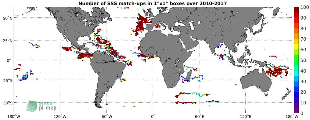
Figure 3: Number of SSS match-ups between Surface drifters SSS and the SMOS SSS L3 v2 - Monthly - 0.25 Deg (CATDS-CECOS-IFREMER) SSS product for the SMOS coastal zone (<800km) 60N-60S Pi-MEP region over 1^\circ \times 1^\circ boxes and for the full satellite product period.
