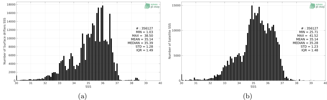
Figure 2: Histograms of SSS from Surface drifters (a) and SMOS SSS L3 v2 - Monthly - 0.25 Deg (CATDS-CECOS-IFREMER) (b) considering all match-up pairs per bins of 0.1 over the SMOS coastal zone (<800km) 60N-60S Pi-MEP region and for the full satellite product period.
