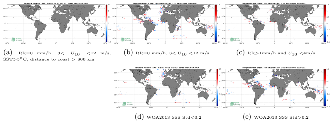
Figure 11: Temporal mean gridded over spatial boxes of size 1^\circ \times 1^\circ of \Delta SSS (SMOS SSS L3 v2 - Monthly - 0.25 Deg (CATDS-CECOS-IFREMER) - Surface drifters) for 5 different subdatasets corresponding to: RR=0 mm/h, 3 < U_{10} < 12 m/s, SST > 5^\circ\text{C} , distance to coast > 800 km (a), RR=0 mm/h, 3 < U_{10} < 12 m/s (b), RR > 1 mm/h and U_{10} < 4 m/s (c), WOA2013 SSS Std < 0.2 (d), WOA2013 SSS Std > 0.2 (e).
