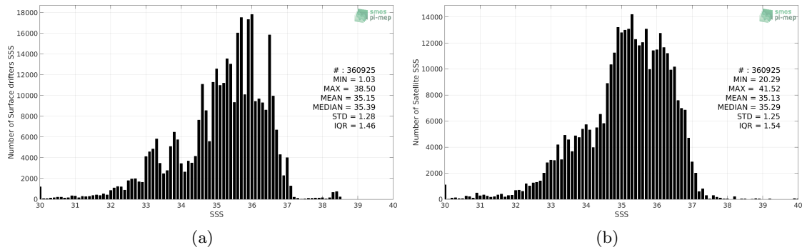
Figure 2: Histograms of SSS from Surface drifters (a) and SMOS SSS L3 v2 - Monthly - 0.25 Deg (CATDS-CECOS-IFREMER) (b) considering all match-up pairs per bins of 0.1 over the SMOS coastal zone (<800km) 60N-60S Pi-MEP region and for the full satellite product period.
