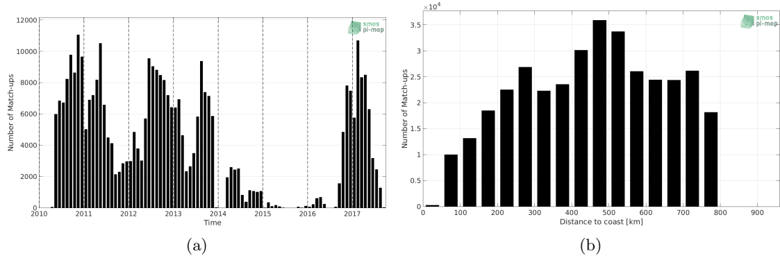
Figure 1: Number of match-ups between Surface drifters and SMOS L3 v2 - Monthly - 0.25 Deg (CATDS-CECOS-IFREMER) SSS as a function of time (a) and as function of the distance to coast (b) over the SMOS coastal zone (<800km) 60N-60S Pi-MEP region and for the full satellite product period.
