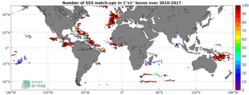
Figure 3: Number of SSS match-ups between Surface drifters SSS and the SMOS L3 v2 - Monthly - 0.25 Deg (CATDS-CECOS-IFREMER) SSS product for the SMOS coastal zone (<800km) 60N-60S Pi-MEP region over 1°x1° boxes and for the full satellite product period.
