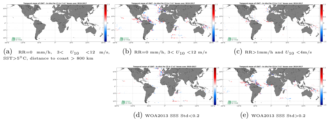
Figure 11: Temporal mean gridded over spatial boxes of size 1^\circ \times 1^\circ of \Delta SSS (SMOS L3 v2 - Monthly - 0.25 Deg (CATDS-CECOS-IFREMER) - Surface drifters) for 5 different subdatasets corresponding to:RR=0 mm/h, 3 < U_{10} < 12 m/s, SST >5^\circ C, distance to coast > 800 km (a), RR=0 mm/h, 3 < U_{10} < 12 m/s (b), RR >1 mm/h and U_{10} < 4 m/s (c), WOA2013 SSS Std <0.2 (d), WOA2013 SSS Std >0.2 (e).
