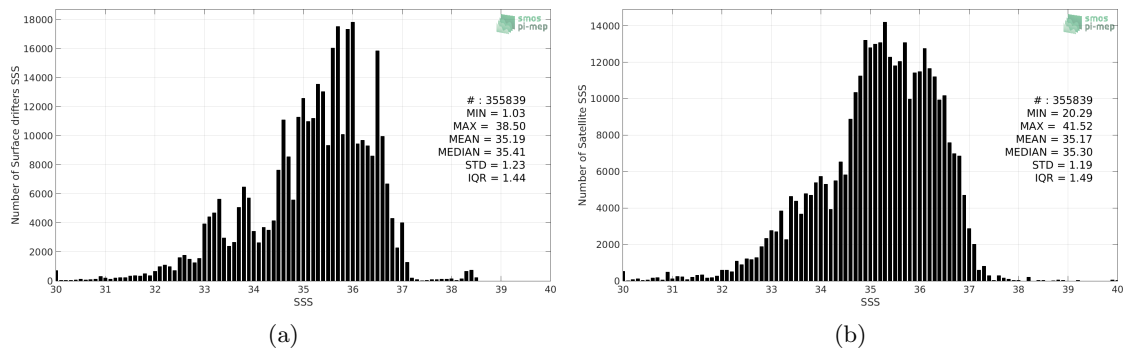
Figure 2: Histograms of SSS from Surface drifters (a) and SMOS L3 v2 - Monthly - 0.25 Deg (CATDS-CECOS-IFREMER) (b) considering all match-up pairs per bins of 0.1 over the SMOS coastal zone (<800km) 60N-60S Pi-MEP region and for the full satellite product period.
