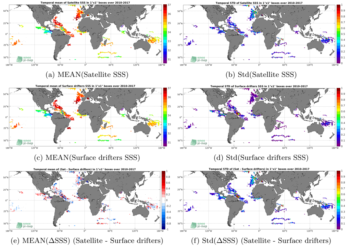
Figure 5: Temporal mean (left) and Std (right) of SSS from SMOS L3 v2 - Monthly - 0.25 Deg (CATDS-CECOS-IFREMER) (top), Surface drifters (middle), and of \Delta SSS (Satellite - Surface drifters). Only match-up pairs are used to generate these maps.
