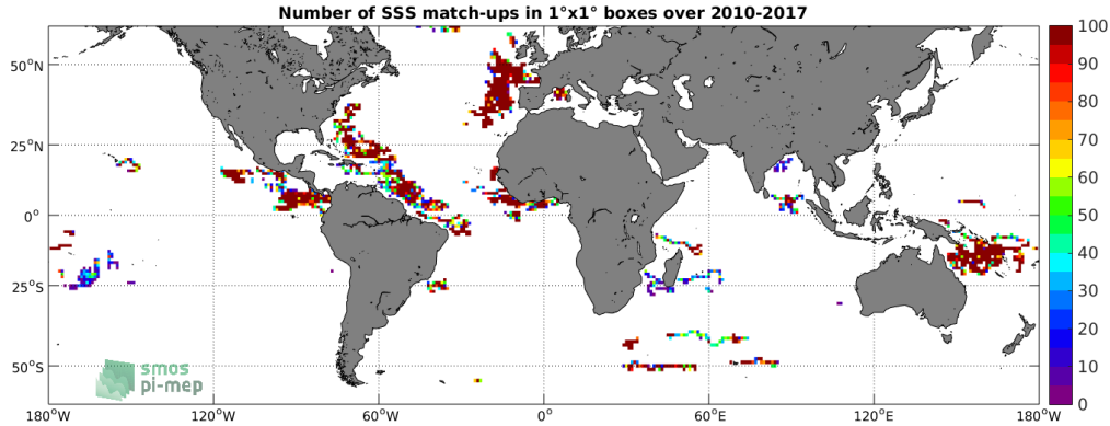
Figure 3: Number of SSS match-ups between Surface drifters SSS and the SMOS-L3-CATDS-IFREMER-CECOS-V2-MONTHLY-0.25DEG SSS product for the SMOS coastal zone ( \approx 800\text{km} ) 60N-60S Pi-MEP region over 1^\circ \times 1^\circ boxes and for the full satellite product period.
