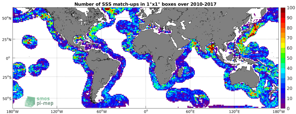
Figure 4: Number of SSS match-ups between Argo SSS and the SMOS SSS L3 v2 - Monthly - 0.25 Deg (CATDS-CECOS-IFREMER) SSS product for the SMOS coastal zone ( <800\text{km} ) 60N-60S Pi-MEP region over 1^\circ \times 1^\circ boxes and for the full satellite product period.
