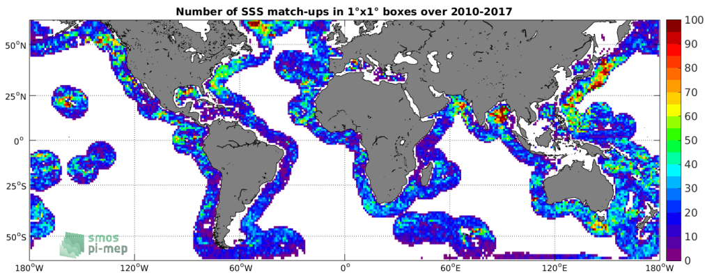
Figure 4: Number of SSS match-ups between Argo SSS and the SMOS-L3-CATDS-IFREMER-CECOS-V2-MONTHLY-0.25DEG SSS product for the SMOS coastal zone ( \approx 800\text{km} ) 60N-60S Pi-MEP region over 1^\circ \times 1^\circ boxes and for the full satellite product period.
