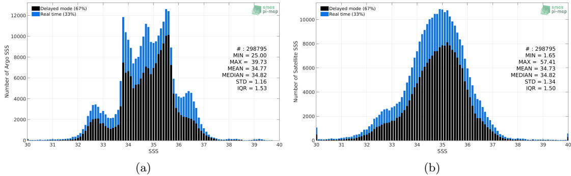
Figure 2: Histograms of SSS from Argo (a) and SMOS-L3-CATDS-IFREMER-CECOS-V2-MONTHLY-0.25DEG (b) considering all match-up pairs per bins of 0.1 over the SMOS coastal zone ( \approx 800 km) 60N-60S Pi-MEP region and for the full satellite product period.
