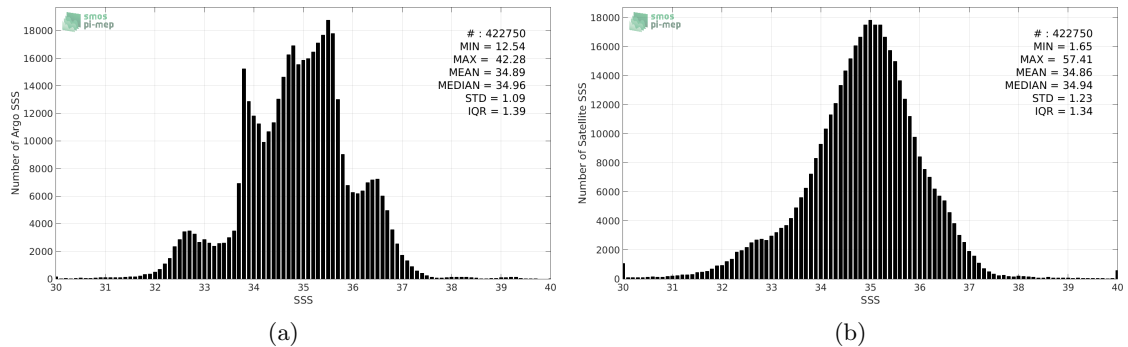
Figure 2: Histograms of SSS from Argo (a) and SMOS-L3-CATDS-IFREMER-CECOS-V2-MONTHLY-0.25DEG (b) considering all match-up pairs per bins of 0.1 over the SMOS coastal zone ( \approx 800\text{km} ) 60N-60S Pi-MEP region and for the full satellite product period.
