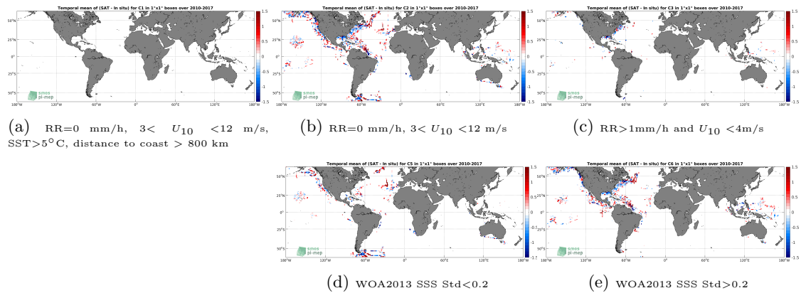
Figure 12: Temporal mean gridded over spatial boxes of size 1^\circ \times 1^\circ of \Delta\text{SSS} (SMOS SSS L3 v2 - Daily - 0.5 Deg (CATDS-CECOS-IFREMER) - TSG (SAMOS)) for 5 different subdatasets corresponding to:RR=0 mm/h, 3 < U_{10} < 12 m/s, SST >5^\circ\text{C} , distance to coast > 800 km (a), RR=0 mm/h, 3 < U_{10} < 12 m/s (b), RR >1 mm/h and U_{10} < 4 m/s (c), WOA2013 SSS Std <0.2 (d), WOA2013 SSS Std >0.2 (e).
