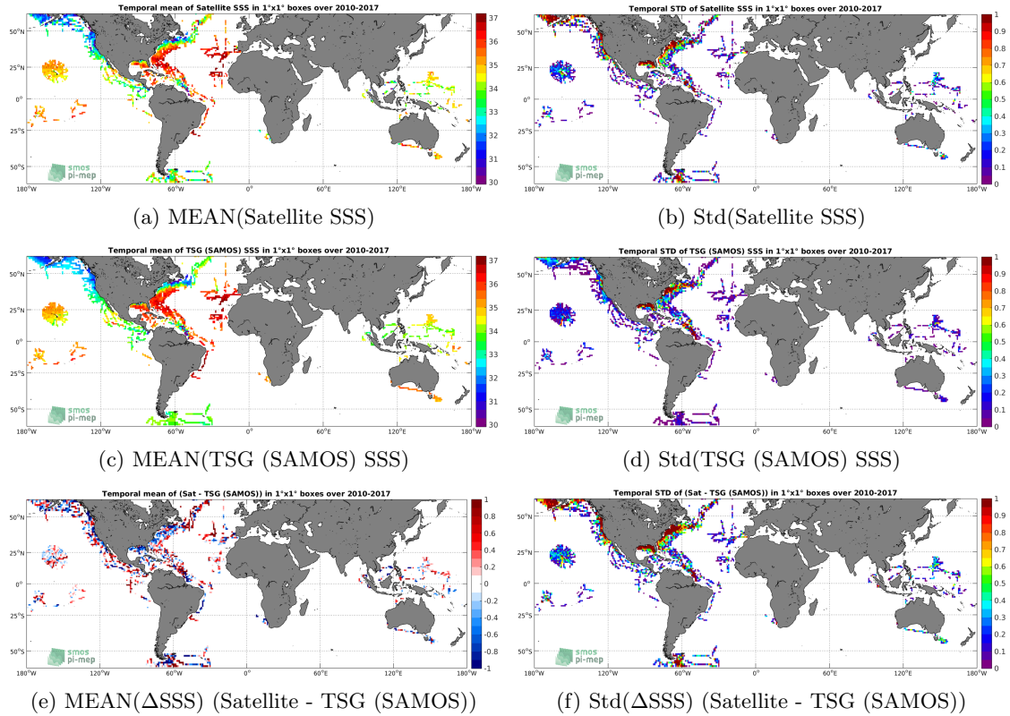
Figure 6: Temporal mean (left) and Std (right) of SSS from SMOS SSS L3 v2 - Daily - 0.5 Deg (CATDS-CECOS-IFREMER) (top), TSG (SAMOS) (middle), and of \Delta SSS (Satellite - TSG (SAMOS)). Only match-up pairs are used to generate these maps.
