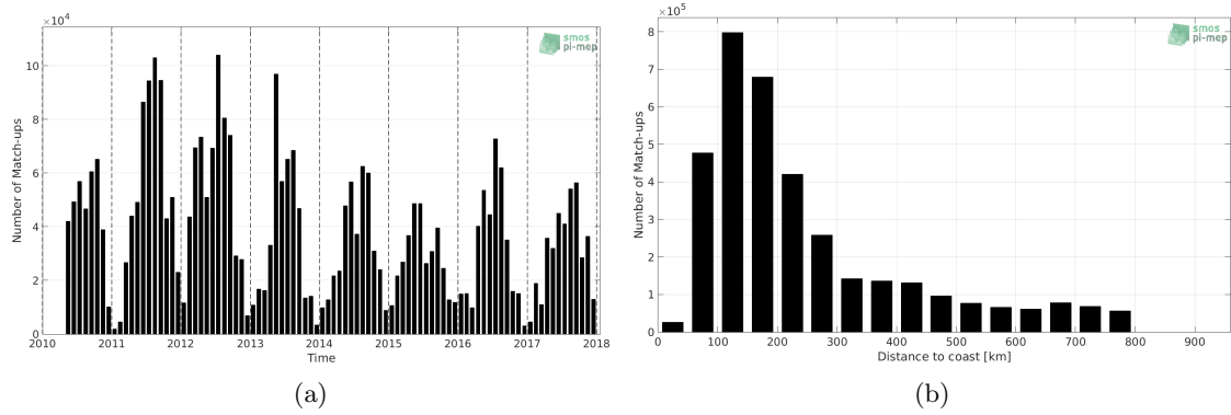
Figure 1: Number of match-ups between TSG (SAMOS) and SMOS SSS L3 v2 - Daily - 0.5 Deg (CATDS-CECOS-IFREMER) SSS as a function of time (a) and as function of the distance to coast (b) over the SMOS coastal zone (<800km) 60N-60S Pi-MEP region and for the full satellite product period.
