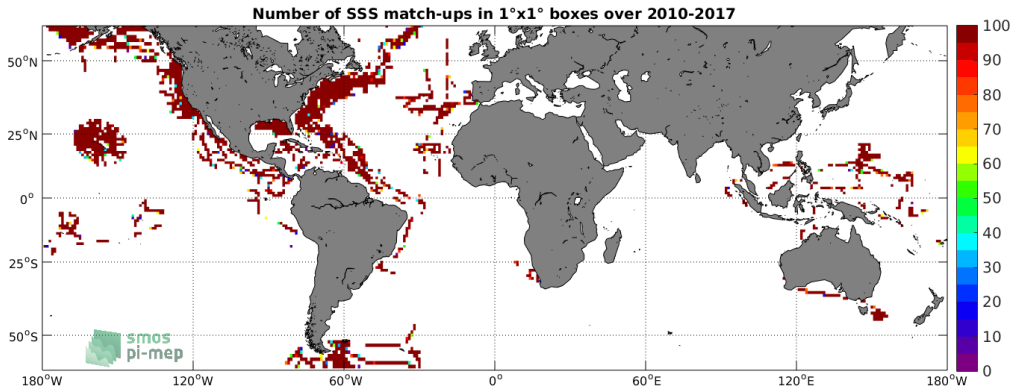
Figure 4: Number of SSS match-ups between TSG (SAMOS) SSS and the SMOS SSS L3 v2 - Daily - 0.5 Deg (CATDS-CECOS-IFREMER) SSS product for the SMOS coastal zone (<800km) 60N-60S Pi-MEP region over 1^\circ \times 1^\circ boxes and for the full satellite product period.
