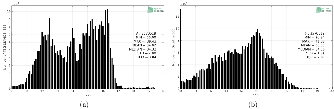
Figure 2: Histograms of SSS from TSG (SAMOS) (a) and SMOS SSS L3 v2 - Daily - 0.5 Deg (CATDS-CECOS-IFREMER) (b) considering all match-up pairs per bins of 0.1 over the SMOS coastal zone (<800km) 60N-60S Pi-MEP region and for the full satellite product period.
