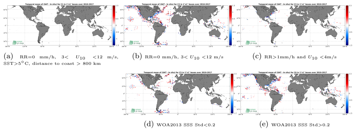
Figure 12: Temporal mean gridded over spatial boxes of size 1^\circ \times 1^\circ of \Delta SSS (SMOS SSS L3 v2 - Daily - 0.5 Deg (CATDS-CECOS-IFREMER) - TSG (SAMOS)) for 5 different subdatasets corresponding to:RR=0 mm/h, 3 < U_{10} < 12 m/s, SST >5^\circ C, distance to coast > 800 km (a), RR=0 mm/h, 3 < U_{10} < 12 m/s (b), RR >1 mm/h and U_{10} < 4 m/s (c), WOA2013 SSS Std <0.2 (d), WOA2013 SSS Std >0.2 (e).
