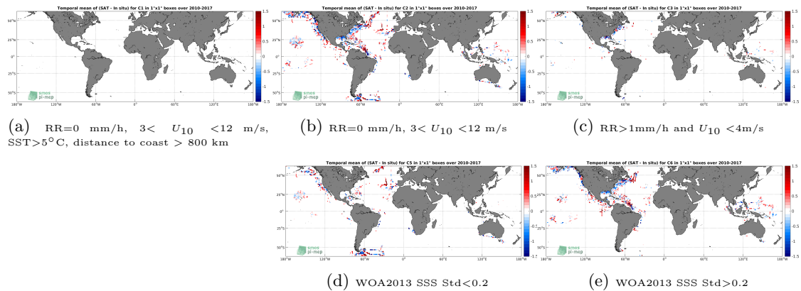
Figure 12: Temporal mean gridded over spatial boxes of size 1^\circ \times 1^\circ of \Delta SSS (SMOS L3 v2 - Daily - 0.5 Deg (CATDS-CECOS-IFREMER) - TSG-SAMOS) for 5 different subdatasets corresponding to:RR=0 mm/h, 3 < U_{10} < 12 m/s, SST >5^\circ C, distance to coast > 800 km (a), RR=0 mm/h, 3 < U_{10} < 12 m/s (b), RR >1 mm/h and U_{10} < 4 m/s (c), WOA2013 SSS Std <0.2 (d), WOA2013 SSS Std >0.2 (e).
