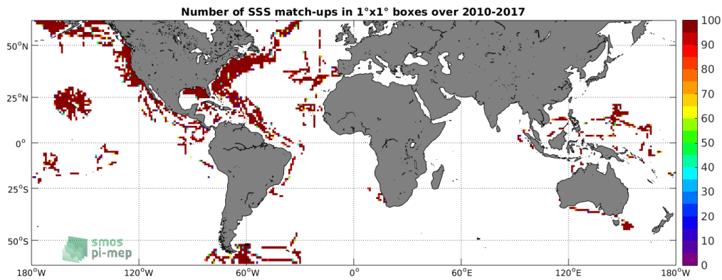
Figure 4: Number of SSS match-ups between TSG-SAMOS SSS and the SMOS L3 v2 - Daily - 0.5 Deg (CATDS-CECOS-IFREMER) SSS product for the SMOS coastal zone (<800km) 60N-60S Pi-MEP region over 1^\circ \times 1^\circ boxes and for the full satellite product period.
