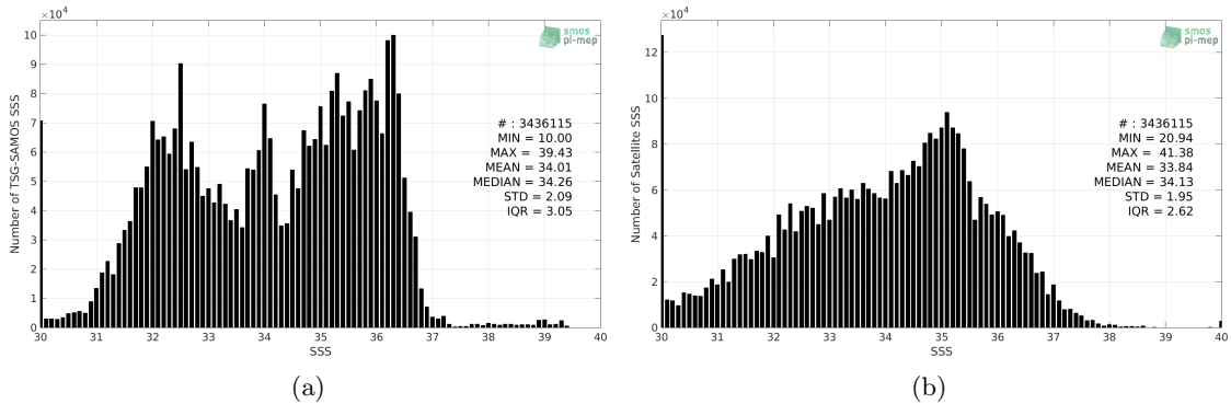
Figure 2: Histograms of SSS from TSG-SAMOS (a) and SMOS L3 v2 - Daily - 0.5 Deg (CATDS-CECOS-IFREMER) (b) considering all match-up pairs per bins of 0.1 over the SMOS coastal zone (<800km) 60N-60S Pi-MEP region and for the full satellite product period.
