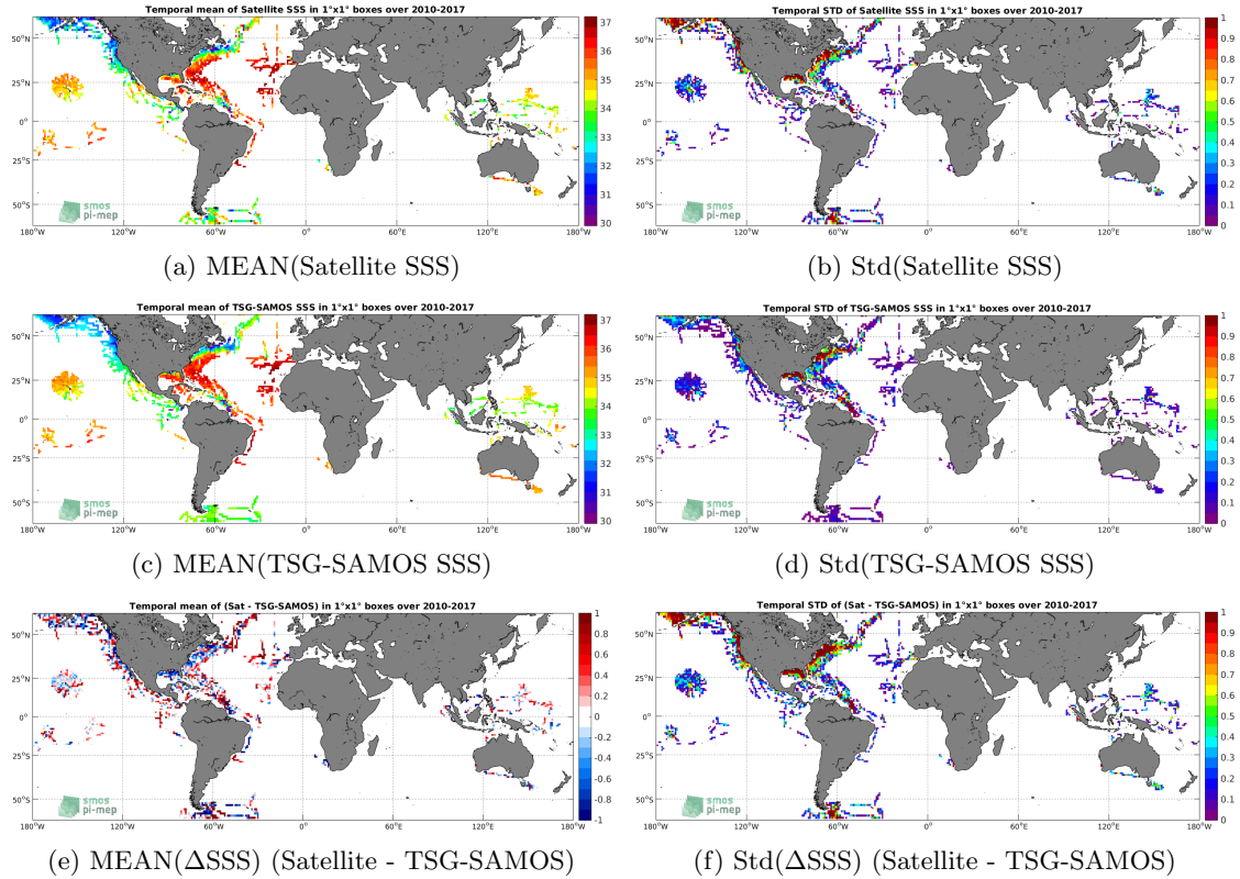
Figure 6: Temporal mean (left) and Std (right) of SSS from SMOS L3 v2 - Daily - 0.5 Deg (CATDS-CECOS-IFREMER) (top), TSG-SAMOS (middle), and of \Delta SSS (Satellite - TSG-SAMOS). Only match-up pairs are used to generate these maps.
