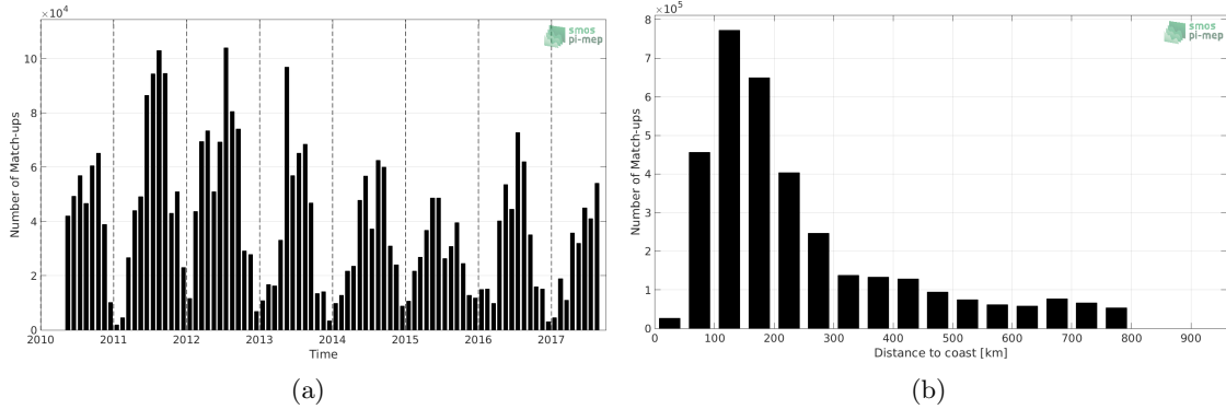
Figure 1: Number of match-ups between TSG-SAMOS and SMOS L3 v2 - Daily - 0.5 Deg (CATDS-CECOS-IFREMER) SSS as a function of time (a) and as function of the distance to coast (b) over the SMOS coastal zone (<800km) 60N-60S Pi-MEP region and for the full satellite product period.
