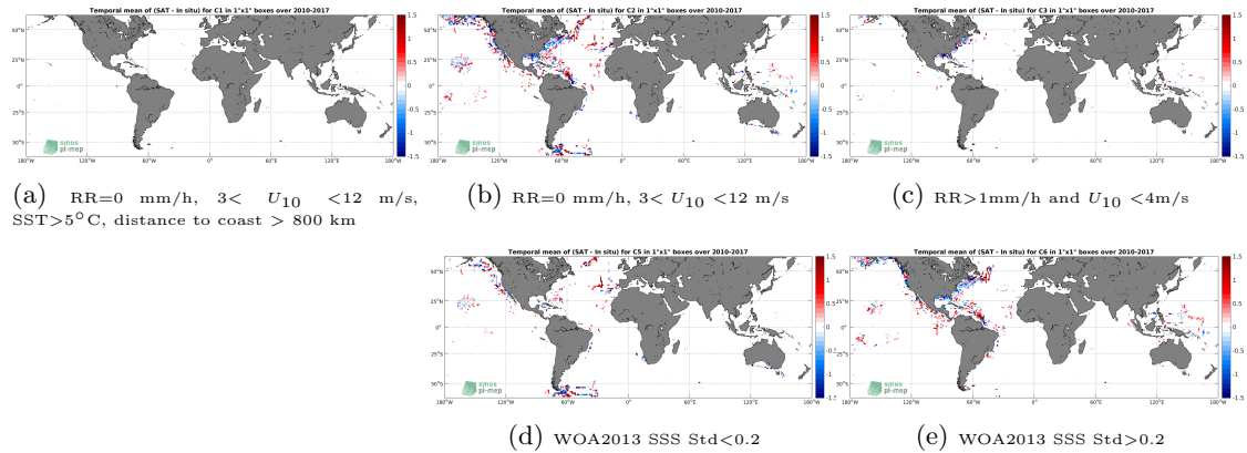
Figure 12: Temporal mean gridded over spatial boxes of size 1^\circ \times 1^\circ of \Delta SSS (SMOS-L3-CATDS-CECOS-IFREMER-V2-1DAY-0.5DEG - TSG-SAMOS) for 5 different subdatasets corresponding to: RR=0 mm/h, 3 < U_{10} < 12 m/s, SST > 5^\circ\text{C} , distance to coast > 800 km (a), RR=0 mm/h, 3 < U_{10} < 12 m/s (b), RR > 1 mm/h and U_{10} < 4 m/s (c), WOA2013 SSS Std < 0.2 (d), WOA2013 SSS Std > 0.2 (e).
