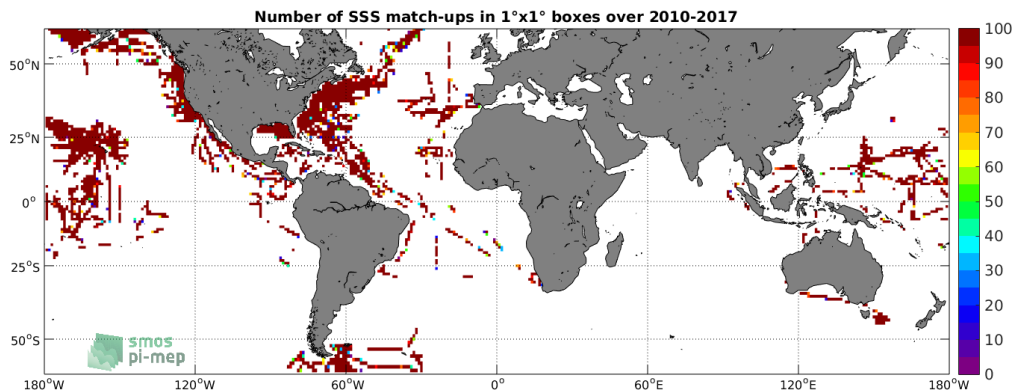
Figure 4: Number of SSS match-ups between TSG-SAMOS SSS and the SMOS-L3-CATDS-CECOS-IFREMER-V2-1DAY-0.5DEG SSS product for the SMOS coastal zone ( \approx 800\text{km} ) 60N-60S Pi-MEP region over 1^\circ \times 1^\circ boxes and for the full satellite product period.
