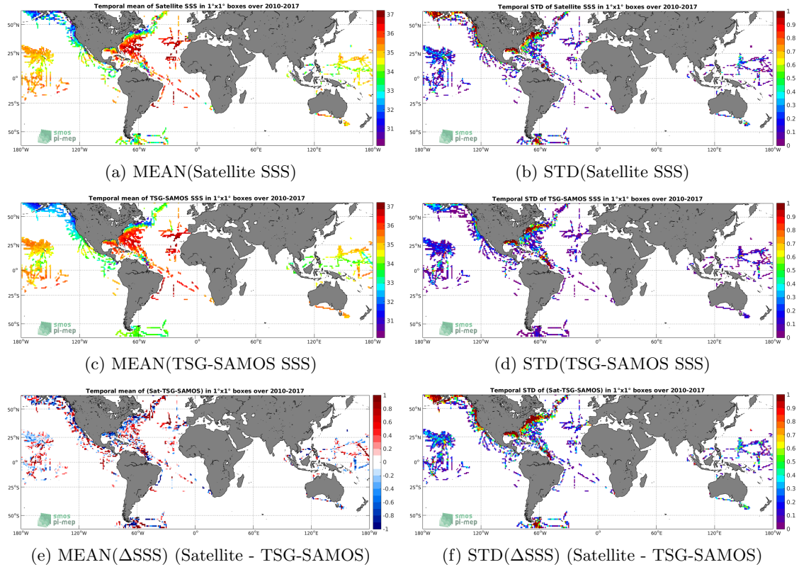
Figure 6: Temporal mean (left) and STD (right) of SSS from SMOS-L3-CATDS-CECOS-IFREMER-V2-1DAY-0.5DEG (top), TSG-SAMOS (middle), and of \Delta SSS (Satellite - TSG-SAMOS). Only match-up pairs are used to generate these maps.
