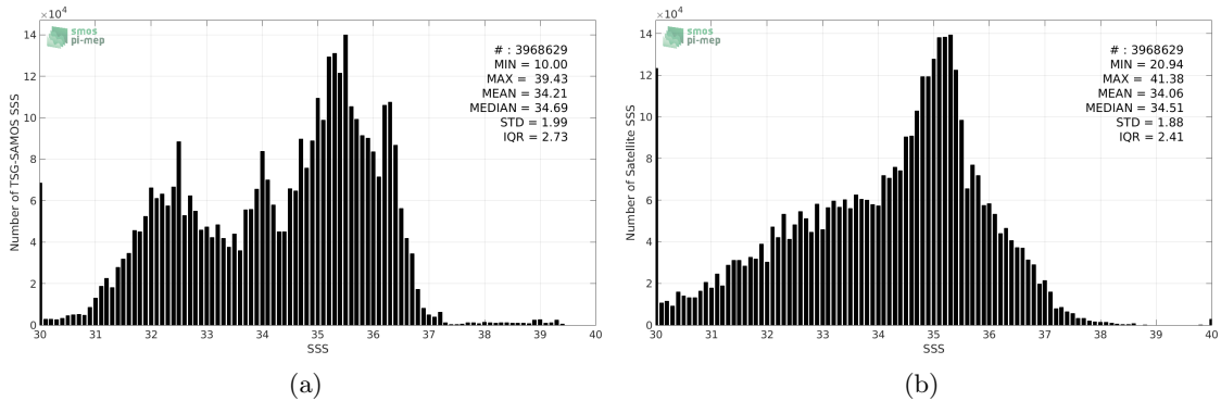
Figure 2: Histograms of SSS from TSG-SAMOS (a) and SMOS-L3-CATDS-CECOS-IFREMER-V2-1DAY-0.5DEG (b) considering all match-up pairs per bins of 0.1 over the SMOS coastal zone ( \geq 800 km) 60N-60S Pi-MEP region and for the full satellite product period.
