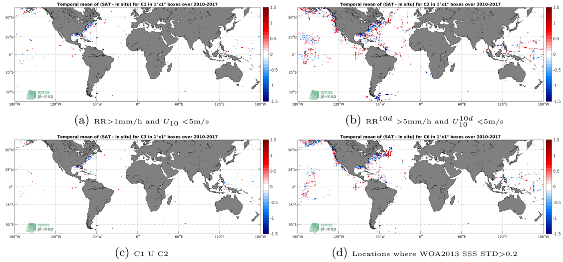
Figure 12: Temporal mean gridded over spatial boxes of size 1^\circ \times 1^\circ of \Delta SSS (SMOS-L3-CATDS-CECOS-IFREMER-V2-1DAY-0.5DEG - TSG-SAMOS) for 4 different subdatasets corresponding to: RR > 1\text{mm/h} and U_{10} < 5\text{m/s} (a), RR^{10d} > 5\text{mm/h} and U_{10}^{10d} < 5\text{m/s} (b), C1 U C2 (c), Locations where WOA2013 SSS STD > 0.2 (d).
