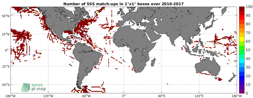
Figure 4: Number of SSS match-ups between TSG-SAMOS SSS and the SMOS-L3-CATDS-CECOS-IFREMER-V2-1DAY-0.5DEG SSS product for the SMOS coastal zone ( \pm 800\text{km} ) 60N-60S Pi-MEP region over 1^\circ \times 1^\circ boxes and for the full satellite product period.
