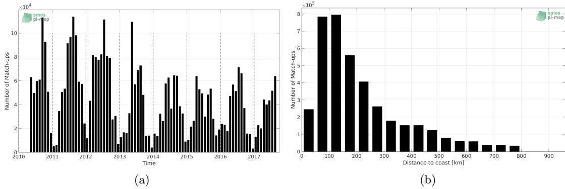
Figure 1: Number of match-ups between TSG-SAMOS and SMOS-L3-CATDS-CECOS-IFREMER-V2-1DAY-0.5DEG SSS as a function of time (a) and as function of the distance to coast (b) over the SMOS coastal zone ( \geq 800 km) 60N-60S Pi-MEP region and for the full satellite product period.
