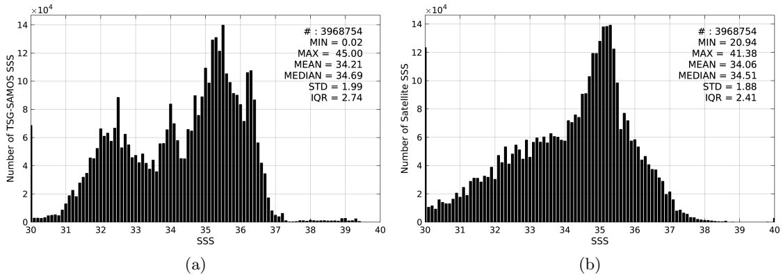
Figure 2: Histograms of SSS from TSG-SAMOS (a) and SMOS-L3-CATDS-CECOS-IFREMER-V2-1DAY-0.5DEG (b) considering all match-up pairs per bins of 0.1 over the SMOS coastal zone ( \leq 800 km) 60N-60S Pi-MEP region and for the full satellite product period.
