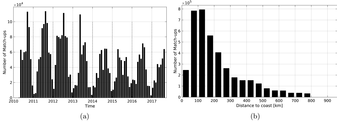
Figure 1: Number of match-ups between TSG-SAMOS and SMOS-L3-CATDS-CECOS-IFREMER-V2-1DAY-0.5DEG SSS as a function of time (a) and as function of the distance to coast (b) over the SMOS coastal zone ( \leq 800 km) 60N-60S Pi-MEP region and for the full satellite product period.
