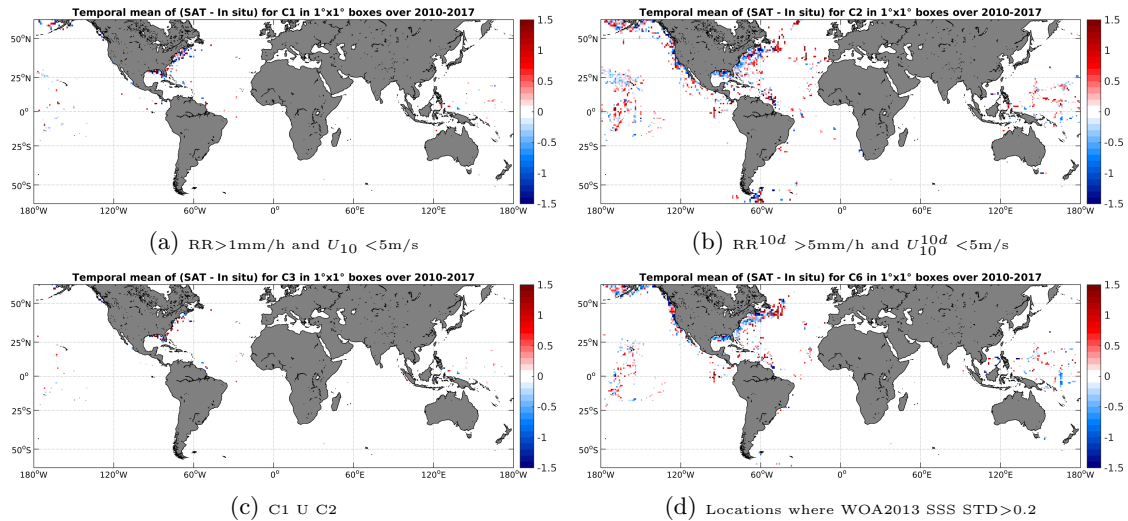
Figure 12: Temporal mean gridded over spatial boxes of size 1^\circ \times 1^\circ of \Delta SSS (SMOS-L3-CATDS-CECOS-IFREMER-V2-1DAY-0.5DEG - TSG-SAMOS) for 4 different subdatasets corresponding to:RR > 1 mm/h and U_{10} < 5 m/s (a), RR 10d > 5 mm/h and U_{10}^{10d} < 5 m/s (b), C1 U C2 (c),Locations where WOA2013 SSS STD > 0.2 (d).
