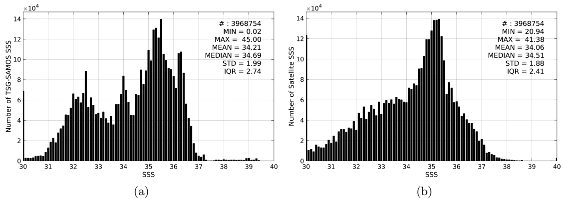
Figure 2: Histograms of SSS from TSG-SAMOS (a) and SMOS-L3-CATDS-CECOS-IFREMER-V2-1DAY-0.5deg (b) considering all match-up pairs per bins of 0.1 over the SMOS coastal zone ( \approx 800\text{km} ) 60N-60S Pi-MEP region and for the full satellite product period.
