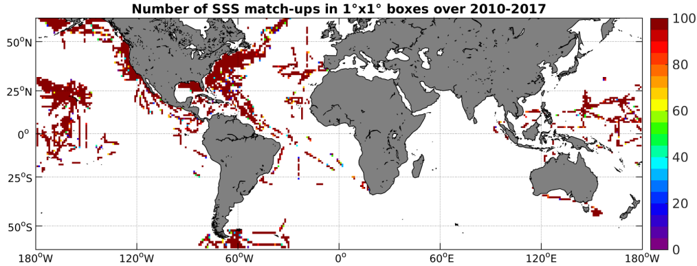
Figure 4: Number of SSS match-ups between TSG-SAMOS SSS and the SMOS-L3-CATDS-CECOS-IFREMER-V2-1DAY-0.5deg SSS product for the SMOS coastal zone ( \geq 800\text{km} ) 60N-60S Pi-MEP region over 1°x1° boxes and for the full satellite product period.
