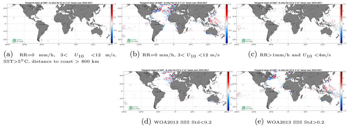
Figure 12: Temporal mean gridded over spatial boxes of size 1^\circ \times 1^\circ of \Delta\text{SSS} (SMOS SSS L3 v2 - Daily - 0.5 Deg (CATDS-CECOS-IFREMER) - TSG (LEGOS-DM)) for 5 different subdatasets corresponding to: RR=0 mm/h, 3 < U_{10} < 12 m/s, SST > 5^\circ\text{C} , distance to coast > 800 km (a), RR=0 mm/h, 3 < U_{10} < 12 m/s (b), RR > 1 mm/h and U_{10} < 4 m/s (c), WOA2013 SSS Std < 0.2 (d), WOA2013 SSS Std > 0.2 (e).
