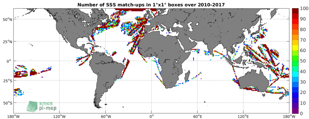
Figure 4: Number of SSS match-ups between TSG (LEGOS-DM) SSS and the SMOS SSS L3 v2 - Daily - 0.5 Deg (CATDS-CECOS-IFREMER) SSS product for the SMOS coastal zone (<800km) 60N-60S Pi-MEP region over 1^\circ \times 1^\circ boxes and for the full satellite product period.
