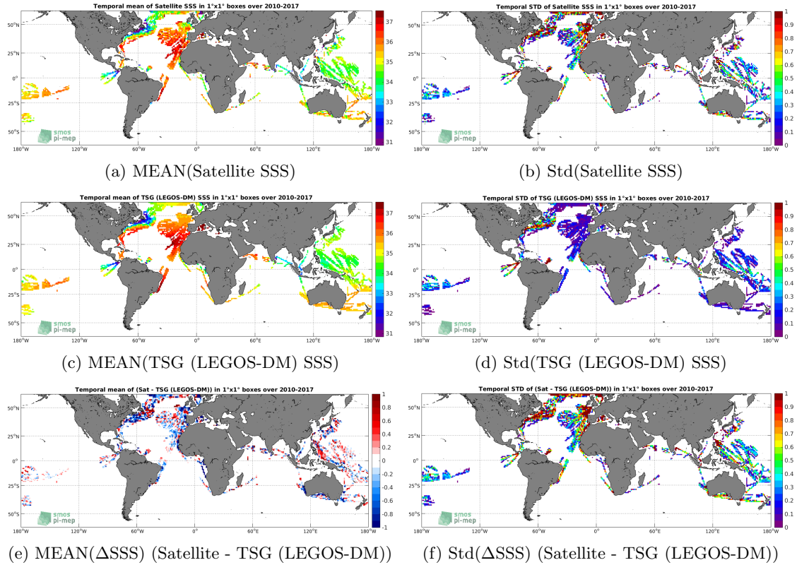
Figure 6: Temporal mean (left) and Std (right) of SSS from SMOS SSS L3 v2 - Daily - 0.5 Deg (CATDS-CECOS-IFREMER) (top), TSG (LEGOS-DM) (middle), and of \Delta SSS (Satellite - TSG (LEGOS-DM)). Only match-up pairs are used to generate these maps.
