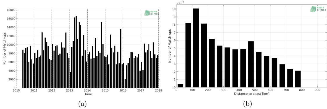
Figure 1: Number of match-ups between TSG (LEGOS-DM) and SMOS SSS L3 v2 - Daily - 0.5 Deg (CATDS-CECOS-IFREMER) SSS as a function of time (a) and as function of the distance to coast (b) over the SMOS coastal zone (<800km) 60N-60S Pi-MEP region and for the full satellite product period.
