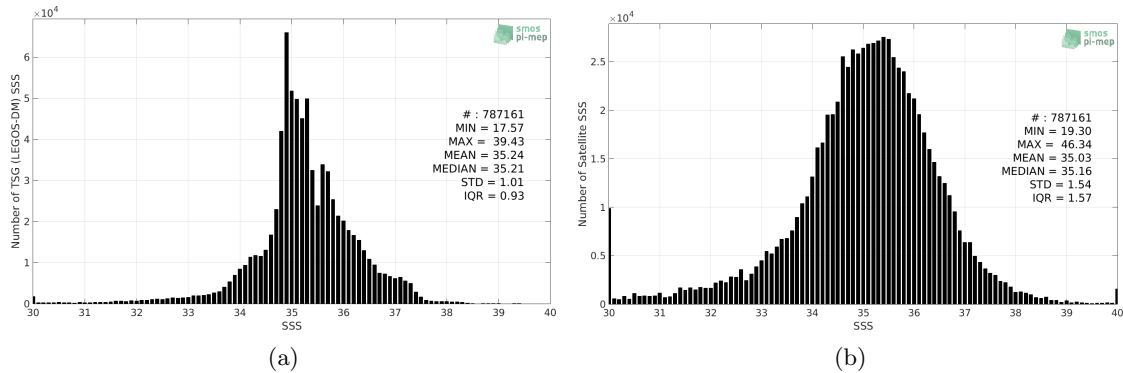
Figure 2: Histograms of SSS from TSG (LEGOS-DM) (a) and SMOS SSS L3 v2 - Daily - 0.5 Deg (CATDS-CECOS-IFREMER) (b) considering all match-up pairs per bins of 0.1 over the SMOS coastal zone (<800km) 60N-60S Pi-MEP region and for the full satellite product period.
